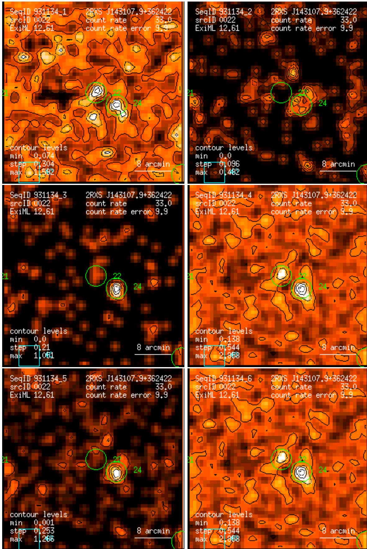
Figure 22: RASS 931134: detection 0022: band rate images, Gaussian filter: (1) PSPC channels 11 – 41, (2) 52 – 90, (3) 91 – 201, (4) 11 – 235, (5) 52 – 201, (6) 11 – 201. Broad band rates in counts/ks. Band rate contour levels in counts/ks/arcmin 2 .
