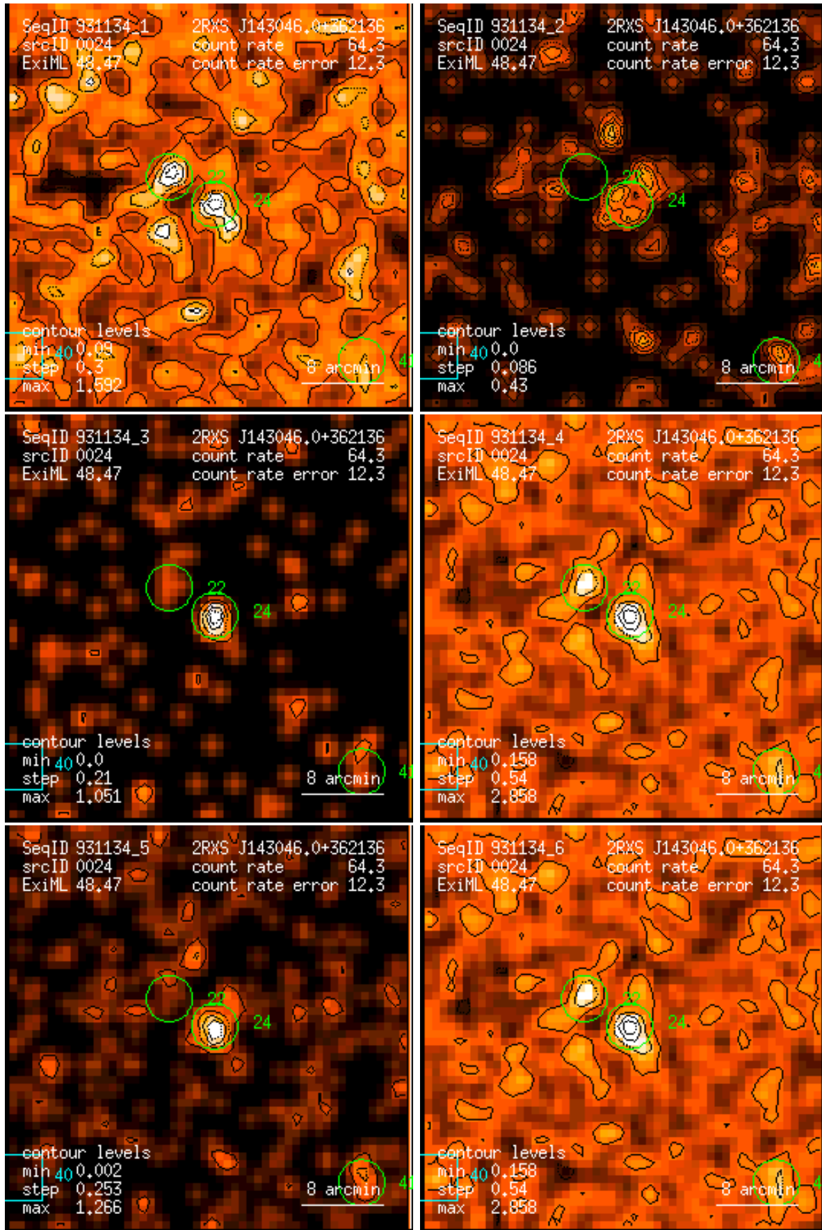
Figure 24: RASS 931134: detection 0024: band rate images, Gaussian filter: (1) PSPC channels 11 – 41, (2) 52 – 90, (3) 91 – 201, (4) 11 – 235, (5) 52 – 201, (6) 11 – 201. Broad band rates in counts/ks. Band rate contour levels in counts/ks/arcmin 2 .
