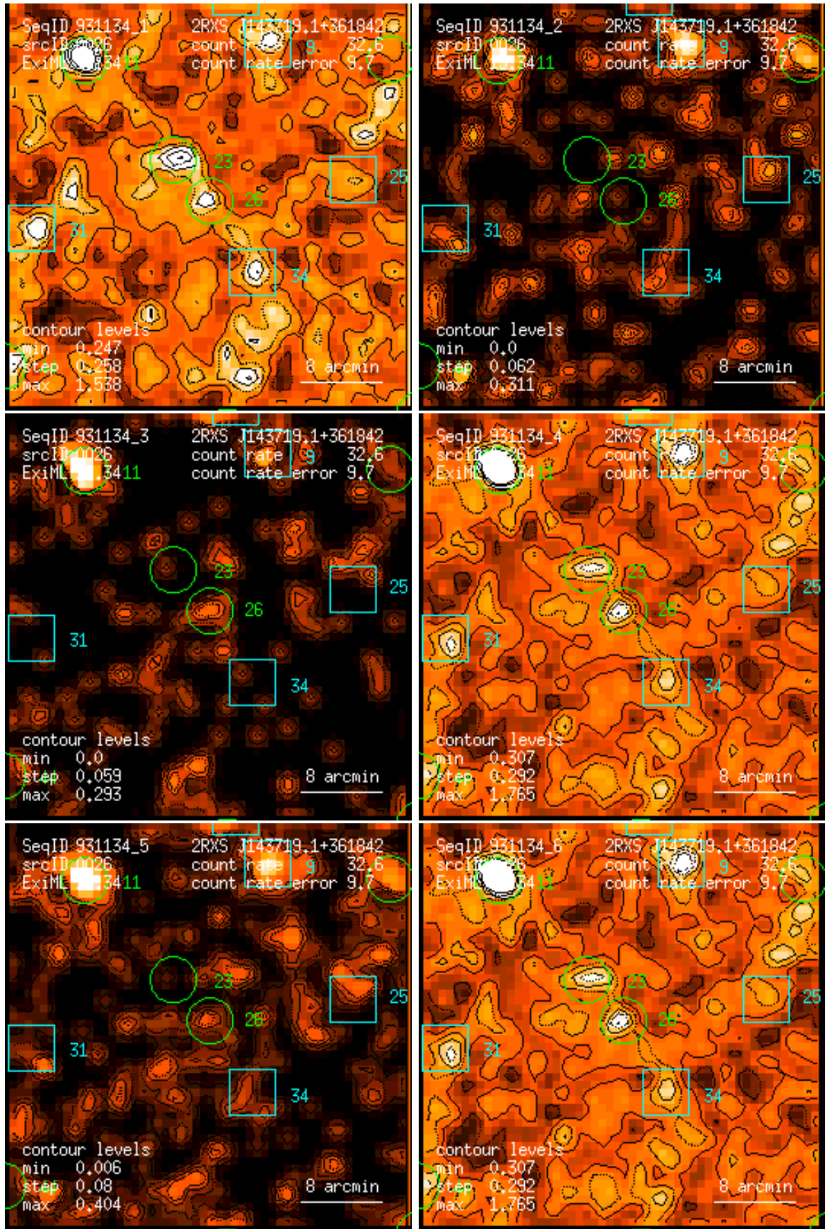
Figure 26: RASS 931134: detection 0026: band rate images, Gaussian filter: (1) PSPC channels 11 – 41, (2) 52 – 90, (3) 91 – 201, (4) 11 – 235, (5) 52 – 201, (6) 11 – 201. Broad band rates in counts/ks. Band rate contour levels in counts/ks/arcmin 2 .
