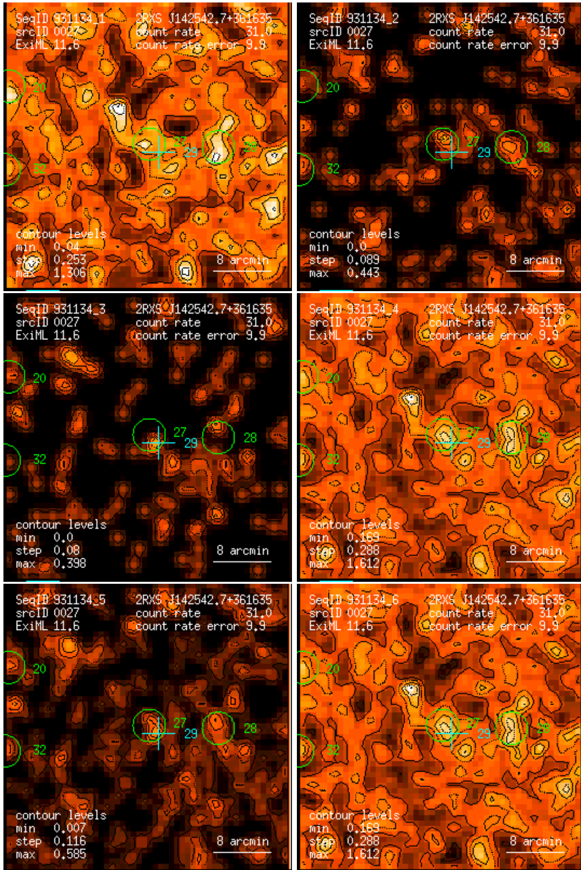
Figure 27: RASS 931134: detection 0027: band rate images, Gaussian filter: (1) PSPC channels 11 – 41, (2) 52 – 90, (3) 91 – 201, (4) 11 – 235, (5) 52 – 201, (6) 11 – 201. Broad band rates in counts/ks. Band rate contour levels in counts/ks/arcmin 2 .
