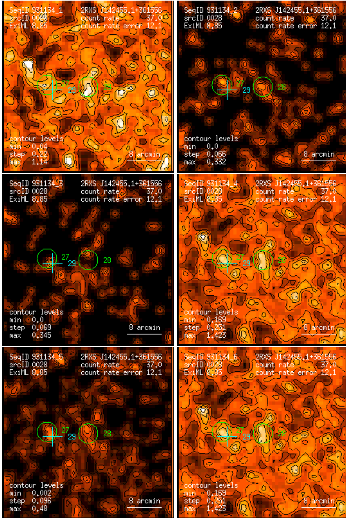
Figure 28: RASS 931134: detection 0028: band rate images, Gaussian filter: (1) PSPC channels 11 – 41, (2) 52 – 90, (3) 91 – 201, (4) 11 – 235, (5) 52 – 201, (6) 11 – 201. Broad band rates in counts/ks. Band rate contour levels in counts/ks/arcmin 2 .
