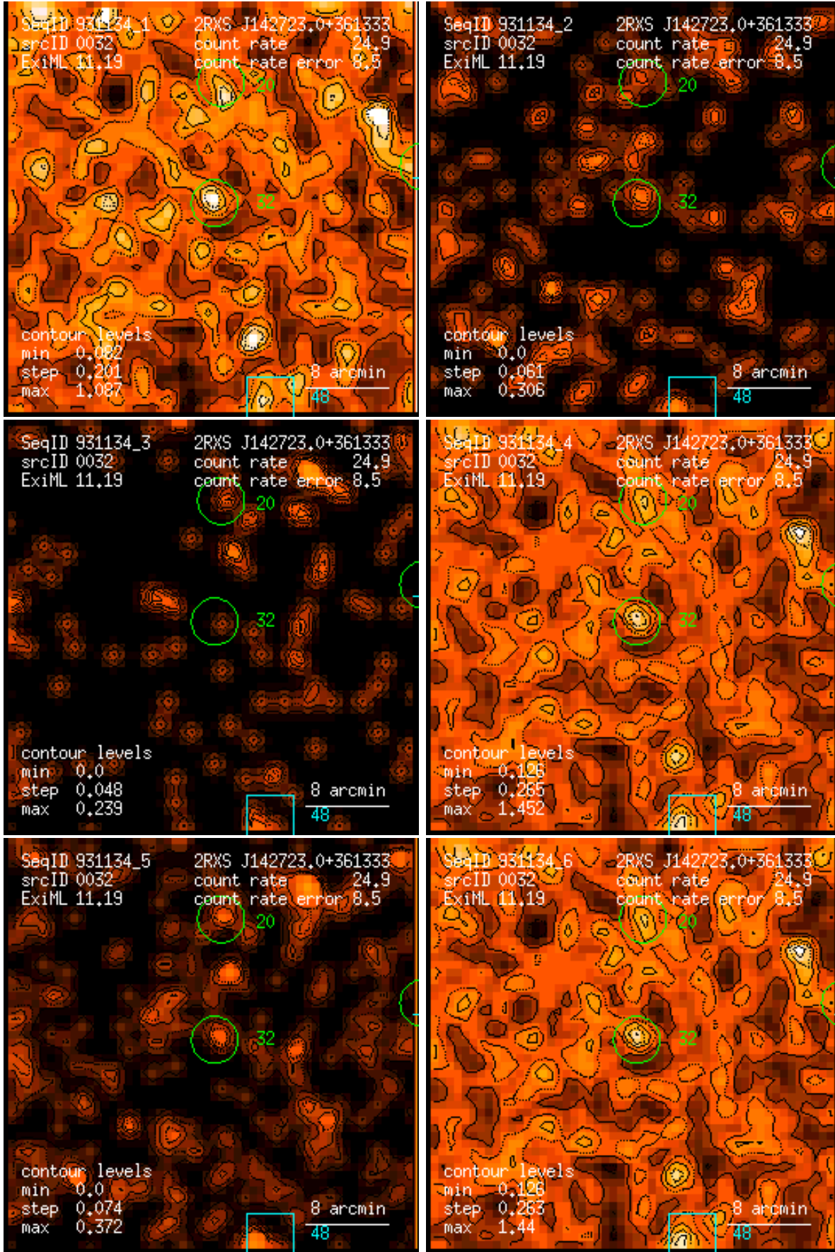
Figure 32: RASS 931134: detection 0032: band rate images, Gaussian filter: (1) PSPC channels 11 – 41, (2) 52 – 90, (3) 91 – 201, (4) 11 – 235, (5) 52 – 201, (6) 11 – 201. Broad band rates in counts/ks. Band rate contour levels in counts/ks/arcmin 2 .
