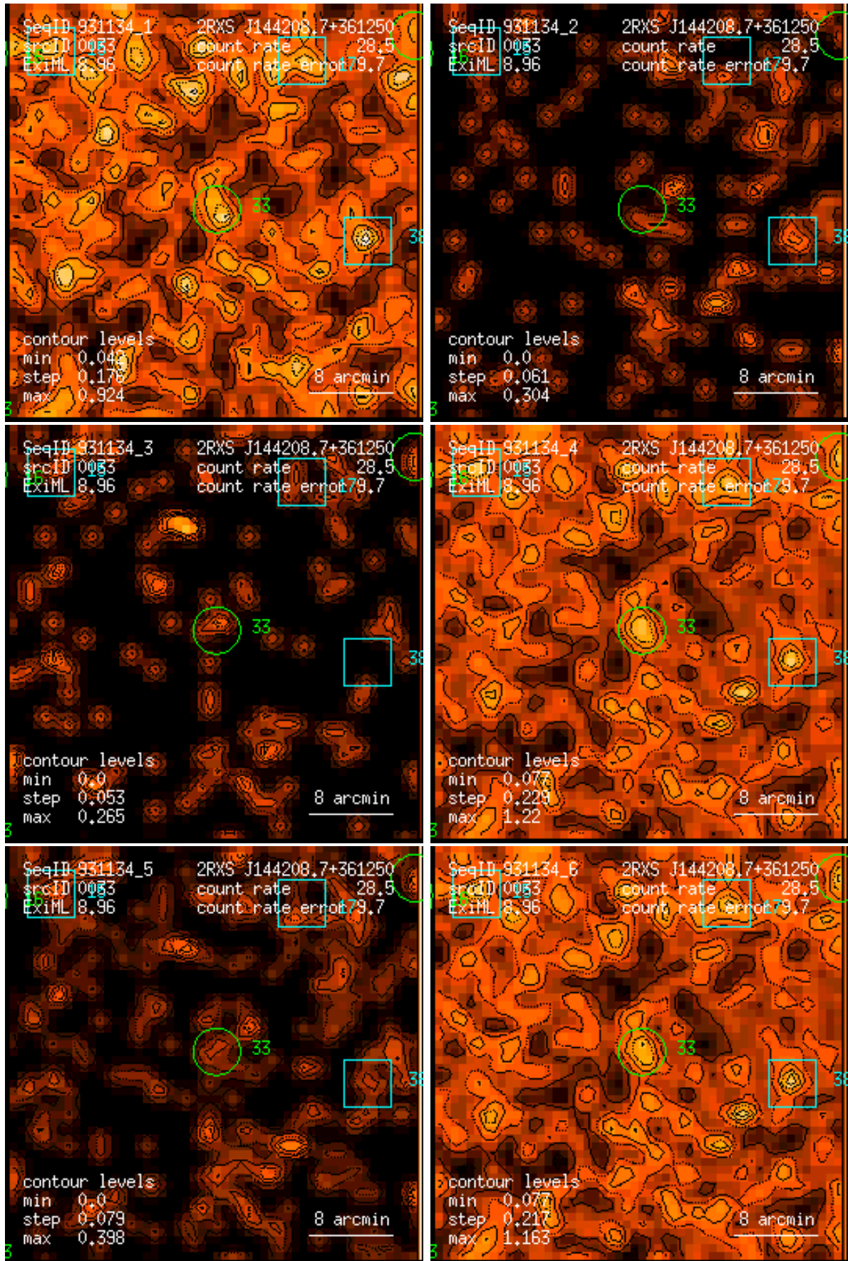
Figure 33: RASS 931134: detection 0033: band rate images, Gaussian filter: (1) PSPC channels 11 – 41, (2) 52 – 90, (3) 91 – 201, (4) 11 – 235, (5) 52 – 201, (6) 11 – 201. Broad band rates in counts/ks. Band rate contour levels in counts/ks/arcmin 2 .
