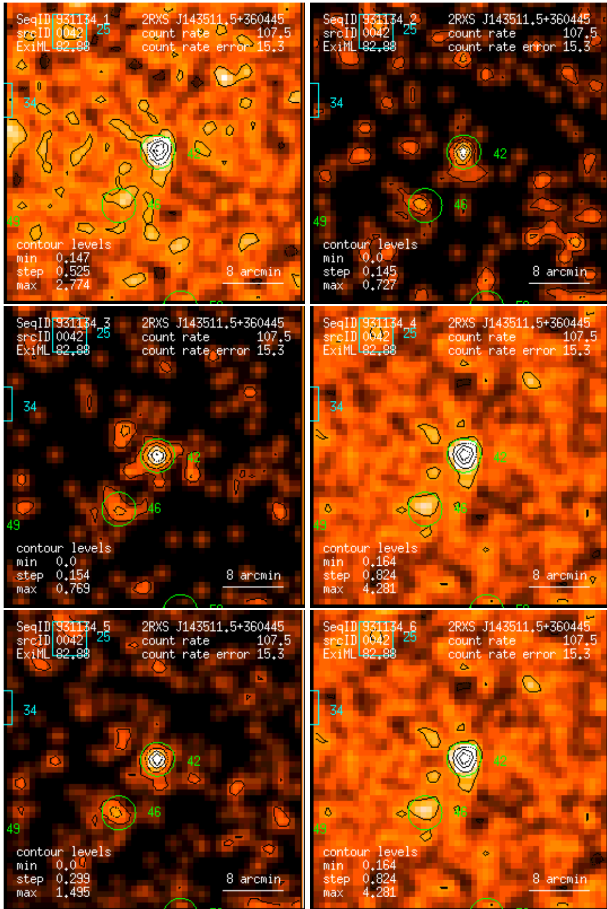
Figure 42: RASS 931134: detection 0042: band rate images, Gaussian filter: (1) PSPC channels 11 – 41, (2) 52 – 90, (3) 91 – 201, (4) 11 – 235, (5) 52 – 201, (6) 11 – 201. Broad band rates in counts/ks. Band rate contour levels in counts/ks/arcmin 2 .
