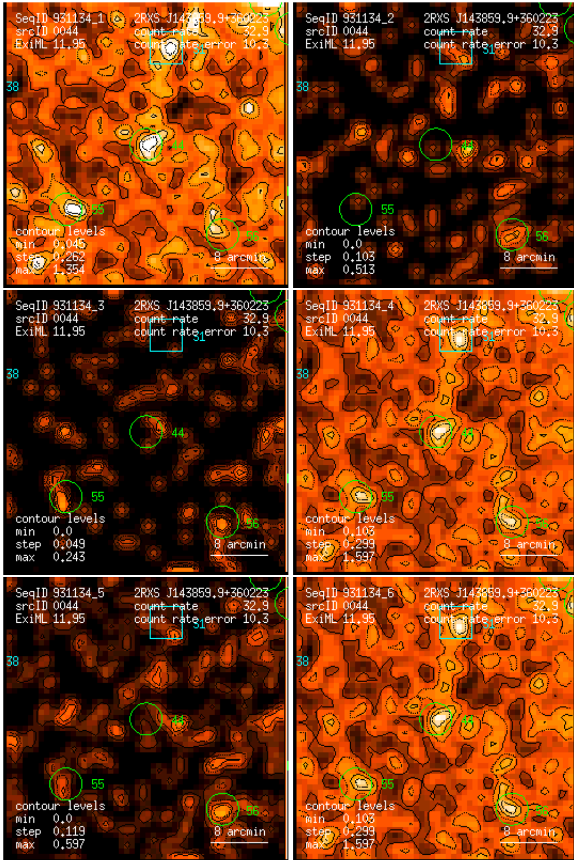
Figure 44: RASS 931134: detection 0044: band rate images, Gaussian filter: (1) PSPC channels 11 – 41, (2) 52 – 90, (3) 91 – 201, (4) 11 – 235, (5) 52 – 201, (6) 11 – 201. Broad band rates in counts/ks. Band rate contour levels in counts/ks/arcmin 2 .
