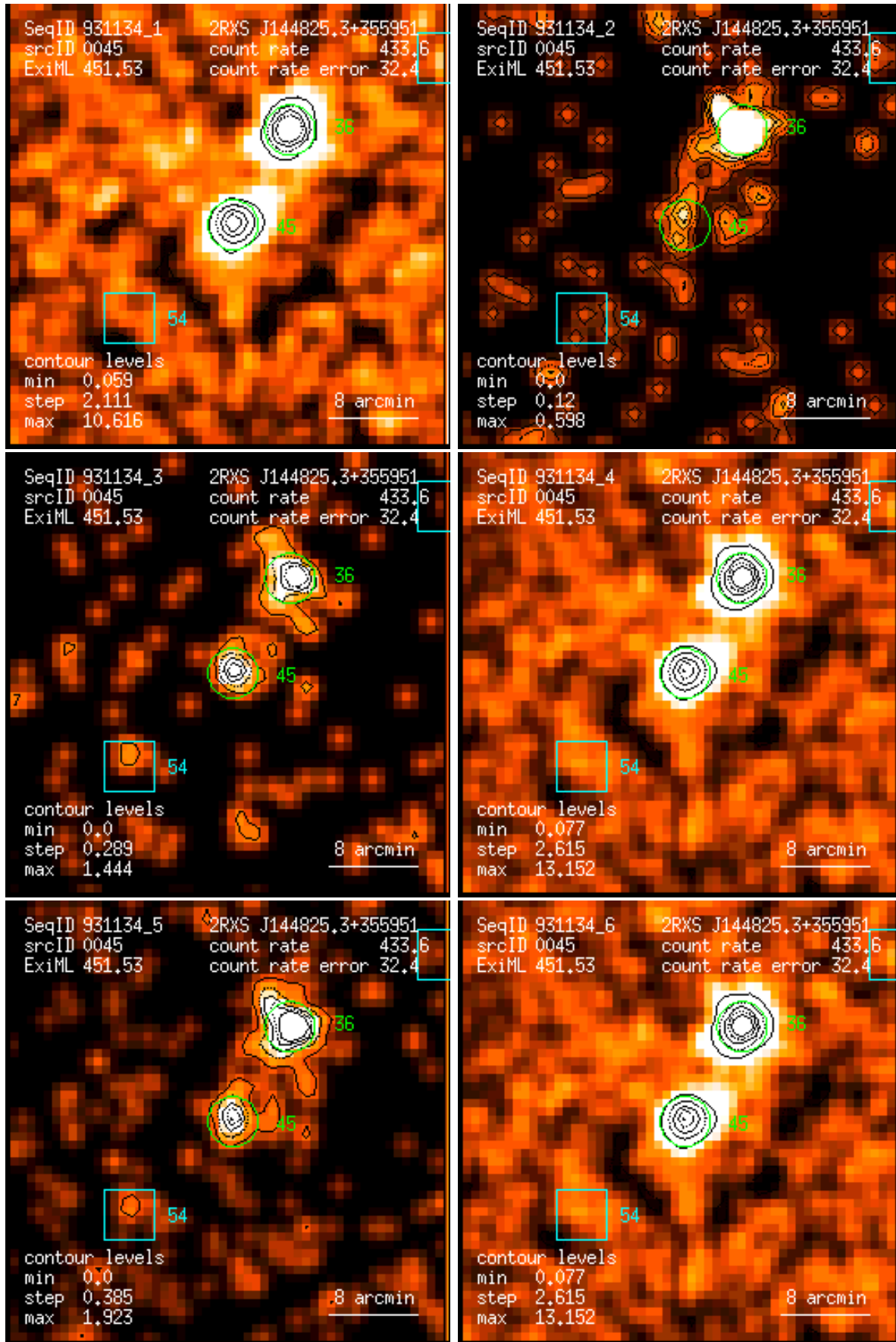
Figure 45: RASS 931134: detection 0045: band rate images, Gaussian filter: (1) PSPC channels 11 – 41, (2) 52 – 90, (3) 91 – 201, (4) 11 – 235, (5) 52 – 201, (6) 11 – 201. Broad band rates in counts/ks. Band rate contour levels in counts/ks/arcmin 2 .
