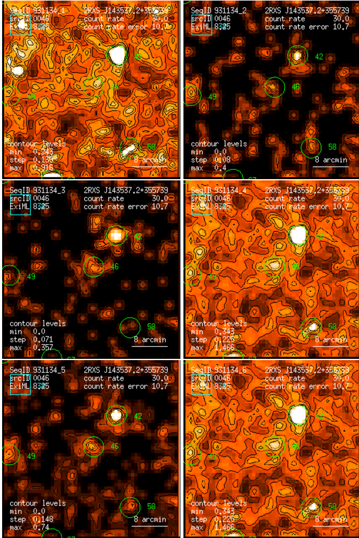
Figure 46: RASS 931134: detection 0046: band rate images, Gaussian filter: (1) PSPC channels 11 – 41, (2) 52 – 90, (3) 91 – 201, (4) 11 – 235, (5) 52 – 201, (6) 11 – 201. Broad band rates in counts/ks. Band rate contour levels in counts/ks/arcmin 2 .
