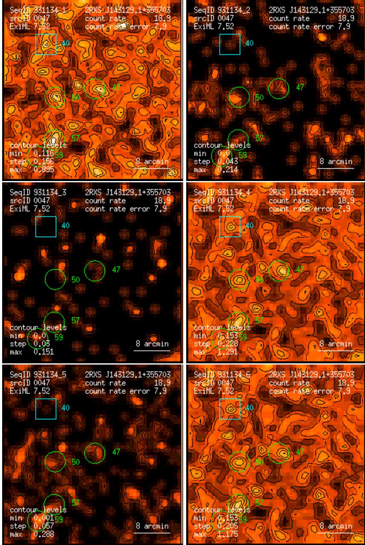
Figure 47: RASS 931134: detection 0047: band rate images, Gaussian filter: (1) PSPC channels 11 – 41, (2) 52 – 90, (3) 91 – 201, (4) 11 – 235, (5) 52 – 201, (6) 11 – 201. Broad band rates in counts/ks. Band rate contour levels in counts/ks/arcmin 2 .
