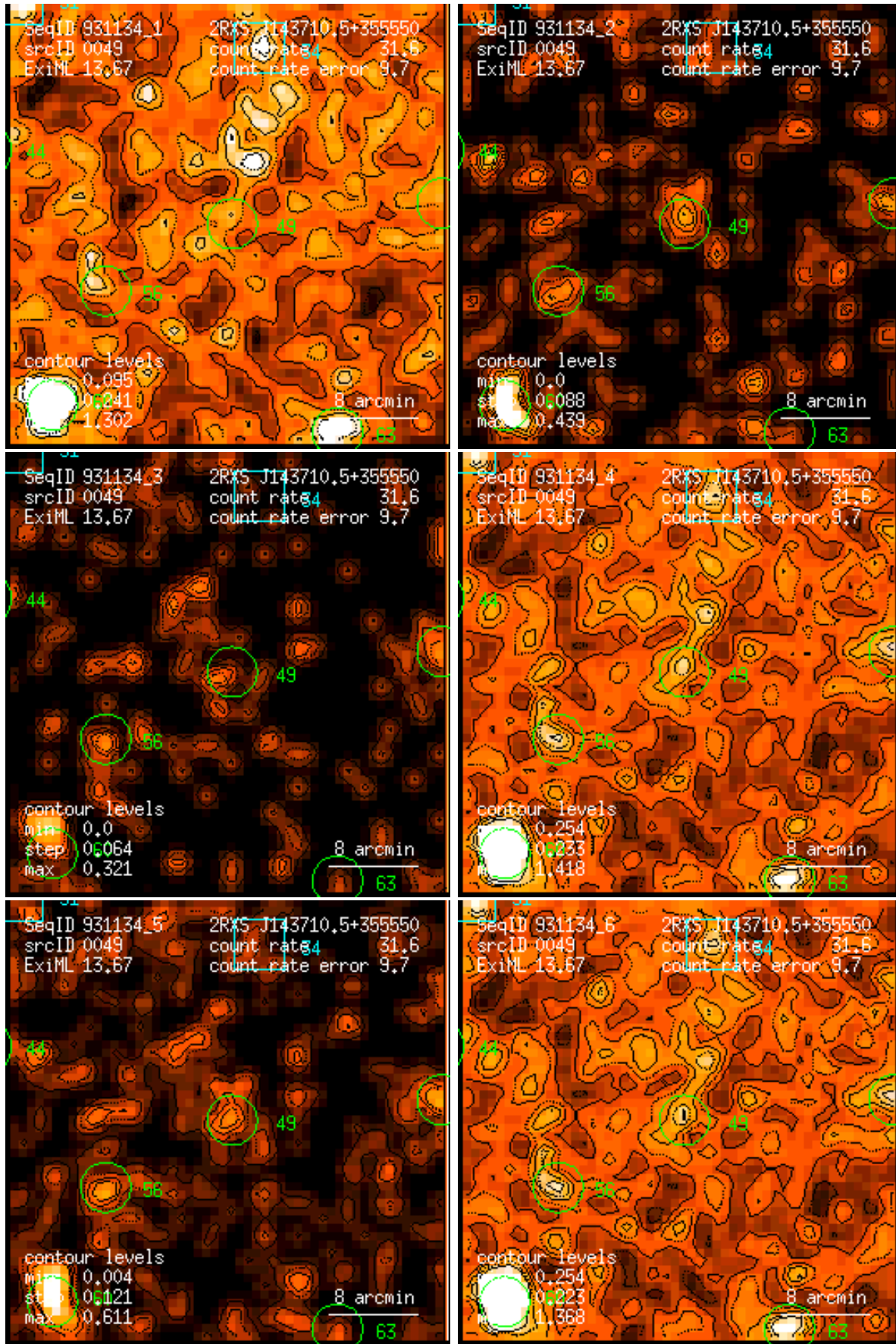
Figure 49: RASS 931134: detection 0049: band rate images, Gaussian filter: (1) PSPC channels 11 – 41, (2) 52 – 90, (3) 91 – 201, (4) 11 – 235, (5) 52 – 201, (6) 11 – 201. Broad band rates in counts/ks. Band rate contour levels in counts/ks/arcmin 2 .
