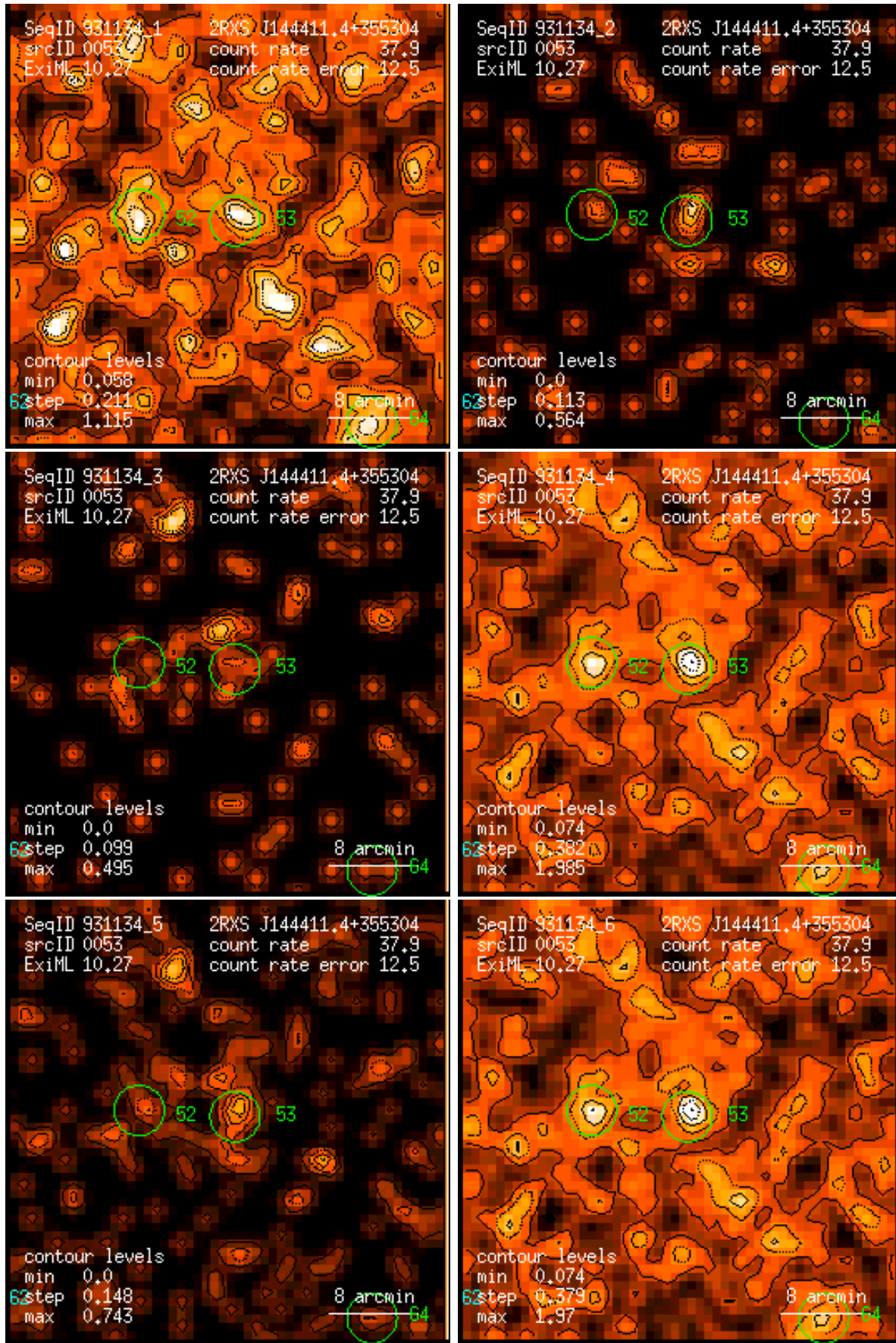
Figure 53: RASS 931134: detection 0053: band rate images, Gaussian filter: (1) PSPC channels 11 – 41, (2) 52 – 90, (3) 91 – 201, (4) 11 – 235, (5) 52 – 201, (6) 11 – 201. Broad band rates in counts/ks. Band rate contour levels in counts/ks/arcmin 2 .
