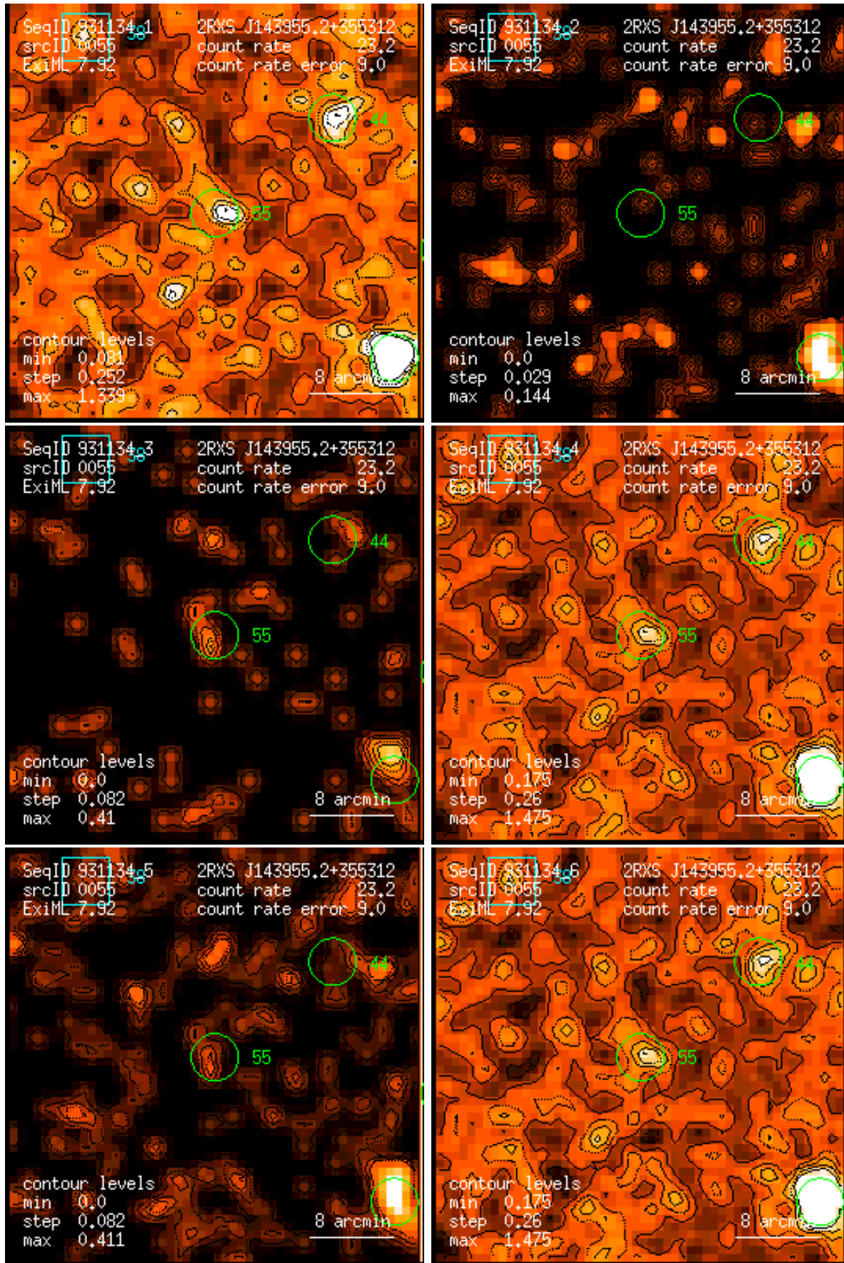
Figure 55: RASS 931134: detection 0055: band rate images, Gaussian filter: (1) PSPC channels 11 – 41, (2) 52 – 90, (3) 91 – 201, (4) 11 – 235, (5) 52 – 201, (6) 11 – 201. Broad band rates in counts/ks. Band rate contour levels in counts/ks/arcmin 2 .
