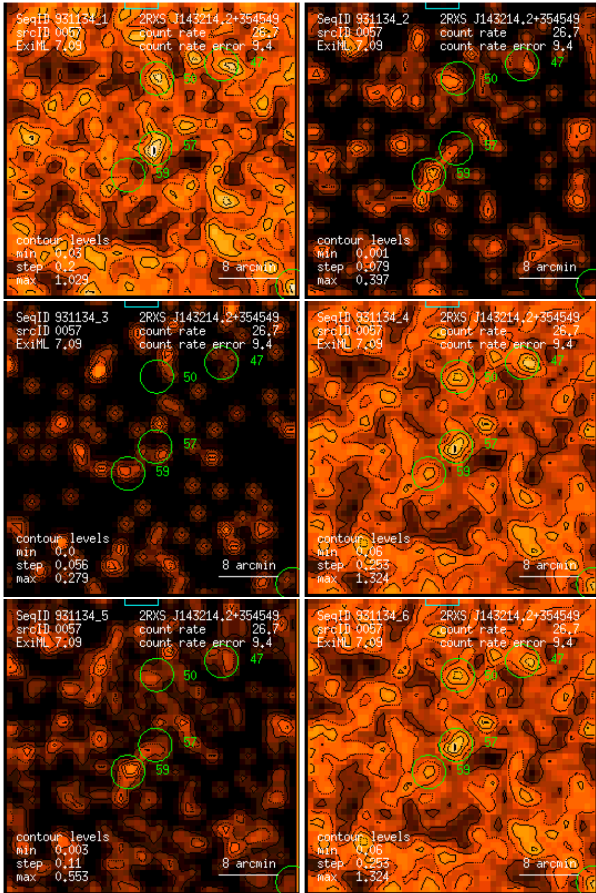
Figure 57: RASS 931134: detection 0057: band rate images, Gaussian filter: (1) PSPC channels 11 – 41, (2) 52 – 90, (3) 91 – 201, (4) 11 – 235, (5) 52 – 201, (6) 11 – 201. Broad band rates in counts/ks. Band rate contour levels in counts/ks/arcmin 2 .
