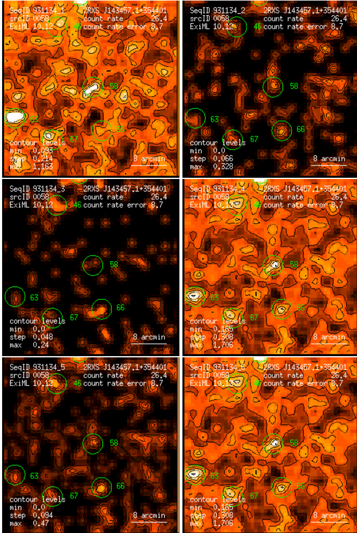
Figure 58: RASS 931134: detection 0058: band rate images, Gaussian filter: (1) PSPC channels 11 – 41, (2) 52 – 90, (3) 91 – 201, (4) 11 – 235, (5) 52 – 201, (6) 11 – 201. Broad band rates in counts/ks. Band rate contour levels in counts/ks/arcmin 2 .
