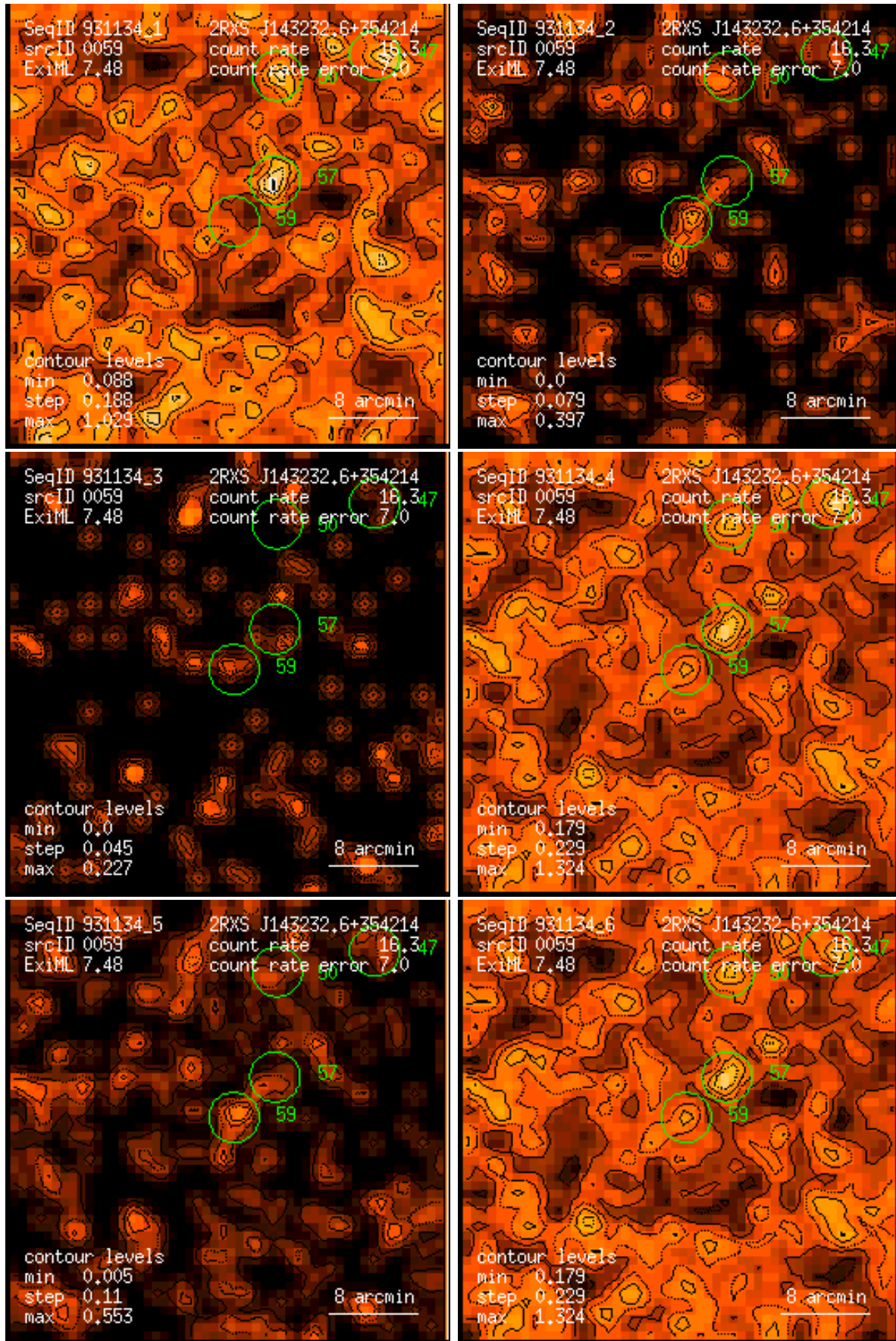
Figure 59: RASS 931134: detection 0059: band rate images, Gaussian filter: (1) PSPC channels 11 – 41, (2) 52 – 90, (3) 91 – 201, (4) 11 – 235, (5) 52 – 201, (6) 11 – 201. Broad band rates in counts/ks. Band rate contour levels in counts/ks/arcmin 2 .
