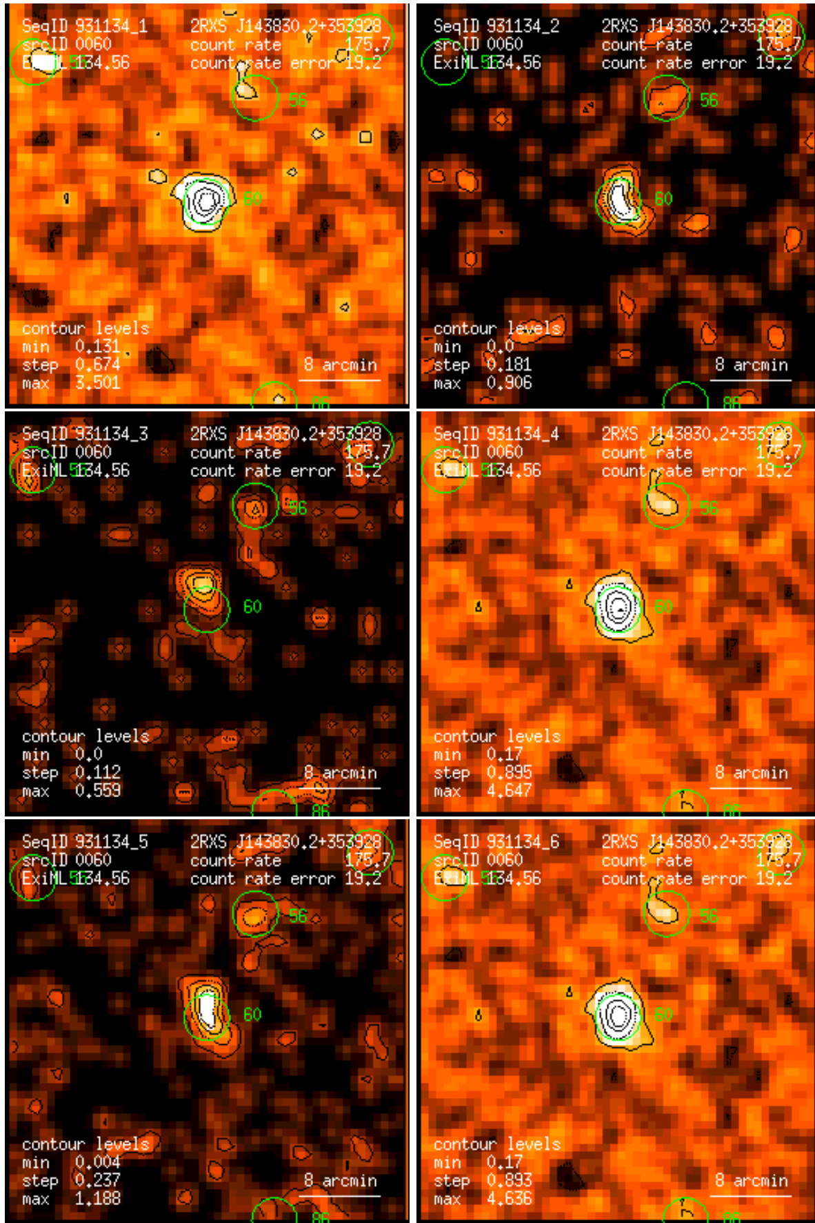
Figure 60: RASS 931134: detection 0060: band rate images, Gaussian filter: (1) PSPC channels 11 – 41, (2) 52 – 90, (3) 91 – 201, (4) 11 – 235, (5) 52 – 201, (6) 11 – 201. Broad band rates in counts/ks. Band rate contour levels in counts/ks/arcmin 2 .
