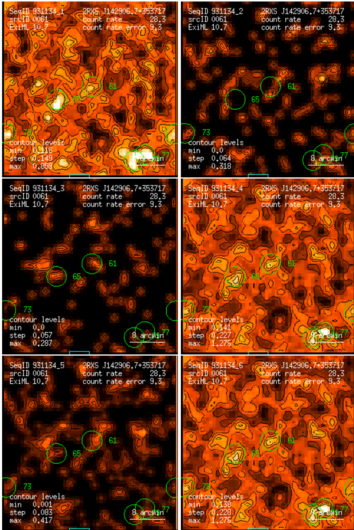
Figure 61: RASS 931134: detection 0061: band rate images, Gaussian filter: (1) PSPC channels 11 – 41, (2) 52 – 90, (3) 91 – 201, (4) 11 – 235, (5) 52 – 201, (6) 11 – 201. Broad band rates in counts/ks. Band rate contour levels in counts/ks/arcmin 2 .
