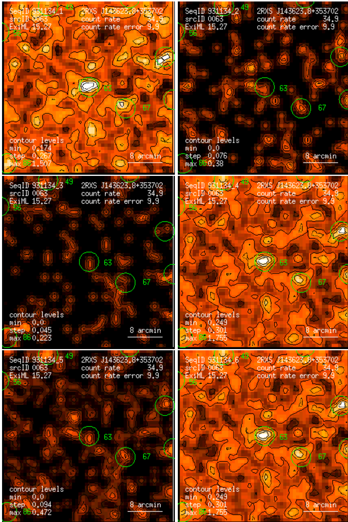
Figure 63: RASS 931134: detection 0063: band rate images, Gaussian filter: (1) PSPC channels 11 – 41, (2) 52 – 90, (3) 91 – 201, (4) 11 – 235, (5) 52 – 201, (6) 11 – 201. Broad band rates in counts/ks. Band rate contour levels in counts/ks/arcmin 2 .
