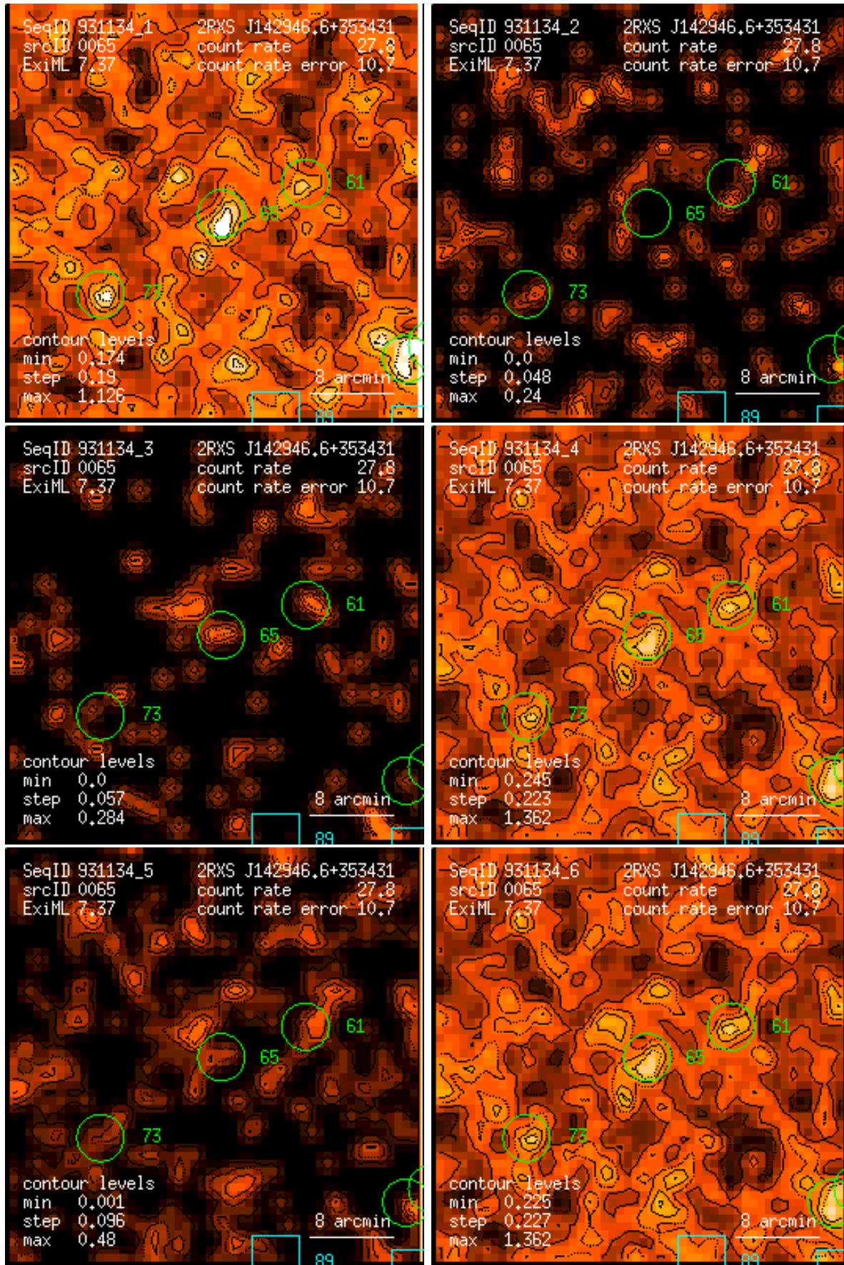
Figure 65: RASS 931134: detection 0065: band rate images, Gaussian filter: (1) PSPC channels 11 – 41, (2) 52 – 90, (3) 91 – 201, (4) 11 – 235, (5) 52 – 201, (6) 11 – 201. Broad band rates in counts/ks. Band rate contour levels in counts/ks/arcmin 2 .
