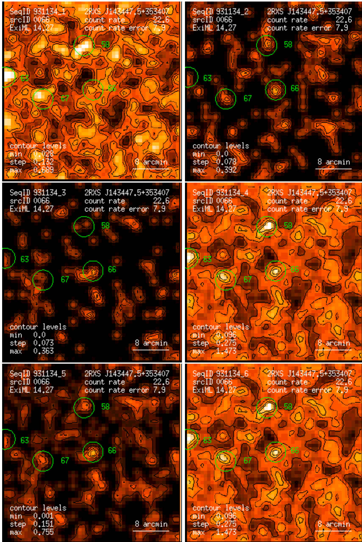
Figure 66: RASS 931134: detection 0066: band rate images, Gaussian filter: (1) PSPC channels 11 – 41, (2) 52 – 90, (3) 91 – 201, (4) 11 – 235, (5) 52 – 201, (6) 11 – 201. Broad band rates in counts/ks. Band rate contour levels in counts/ks/arcmin 2 .
