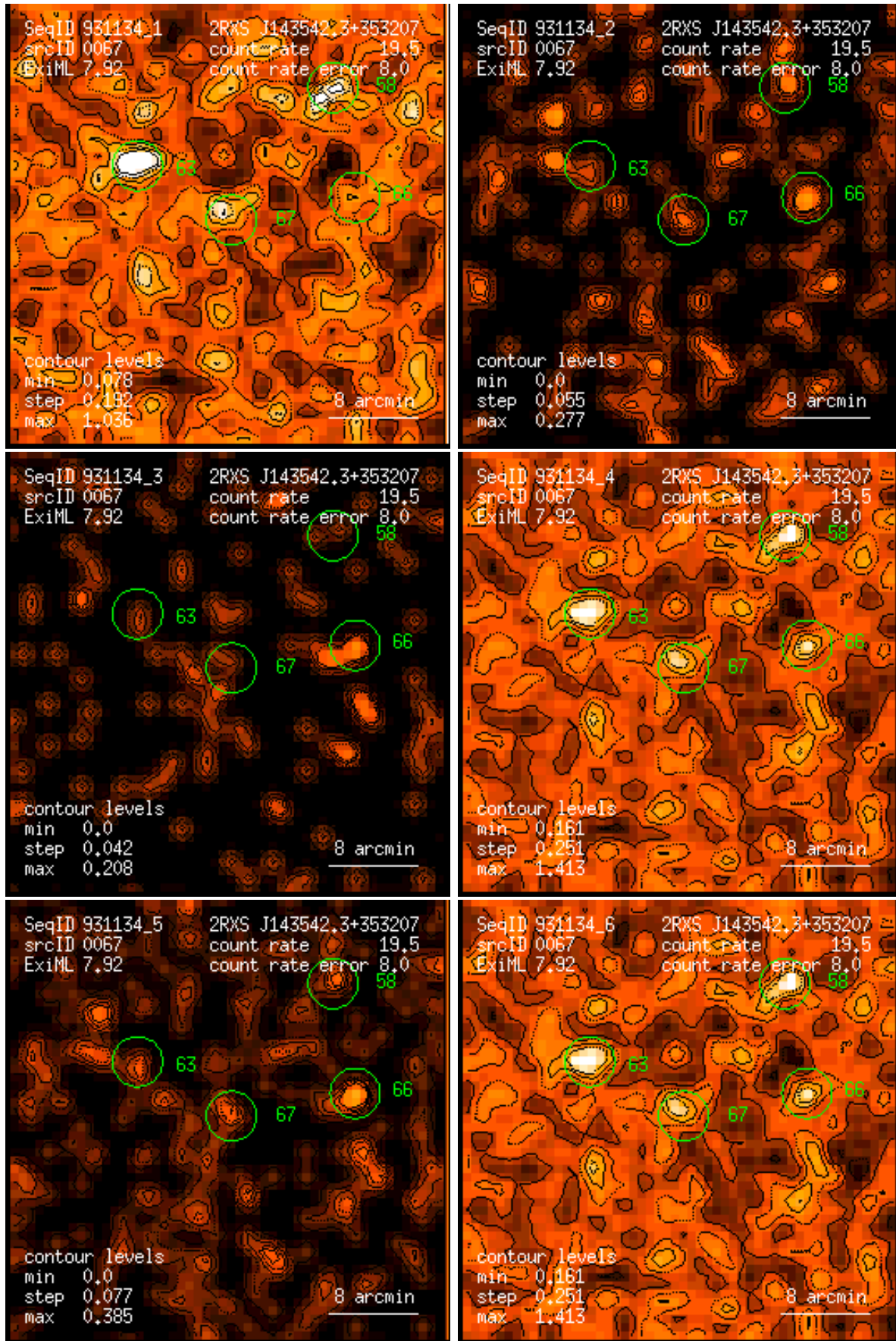
Figure 67: RASS 931134: detection 0067: band rate images, Gaussian filter: (1) PSPC channels 11 – 41, (2) 52 – 90, (3) 91 – 201, (4) 11 – 235, (5) 52 – 201, (6) 11 – 201. Broad band rates in counts/ks. Band rate contour levels in counts/ks/arcmin 2 .
