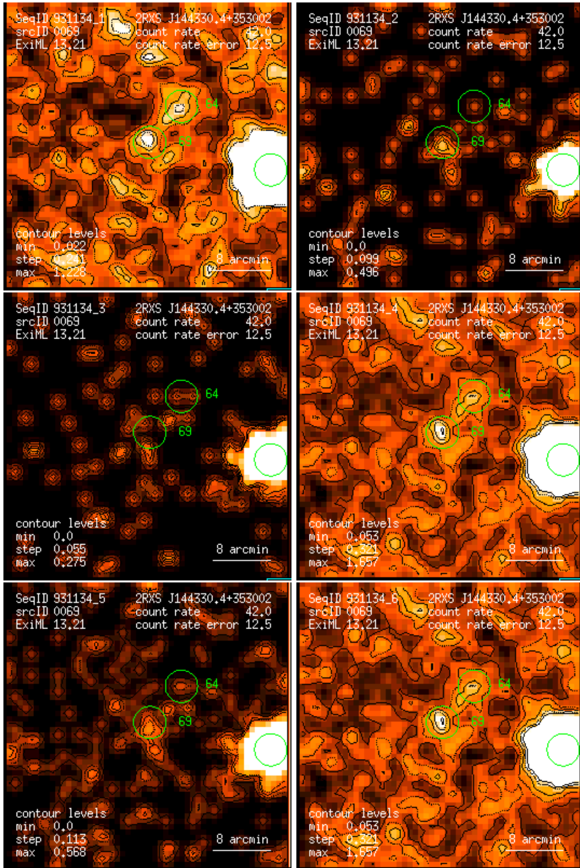
Figure 69: RASS 931134: detection 0069: band rate images, Gaussian filter: (1) PSPC channels 11 – 41, (2) 52 – 90, (3) 91 – 201, (4) 11 – 235, (5) 52 – 201, (6) 11 – 201. Broad band rates in counts/ks. Band rate contour levels in counts/ks/arcmin 2 .
