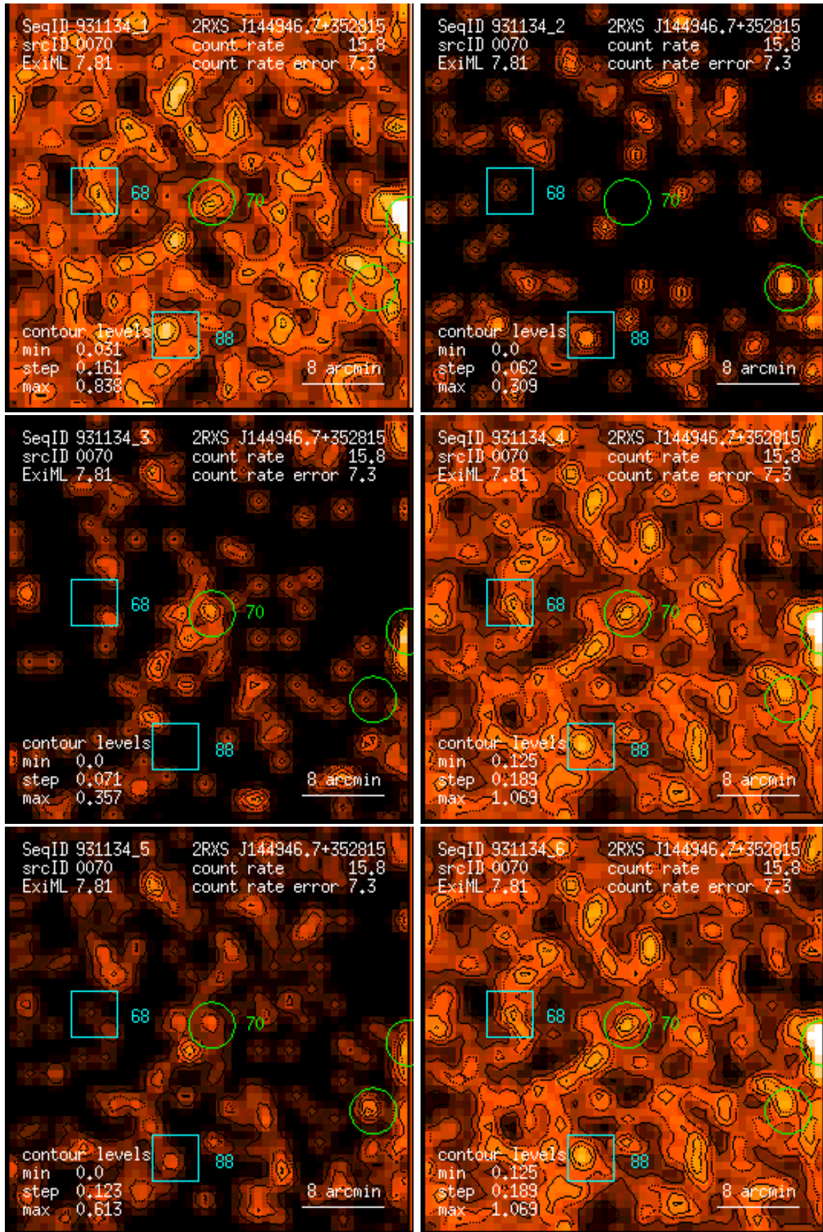
Figure 70: RASS 931134: detection 0070: band rate images, Gaussian filter: (1) PSPC channels 11 – 41, (2) 52 – 90, (3) 91 – 201, (4) 11 – 235, (5) 52 – 201, (6) 11 – 201. Broad band rates in counts/ks. Band rate contour levels in counts/ks/arcmin 2 .
