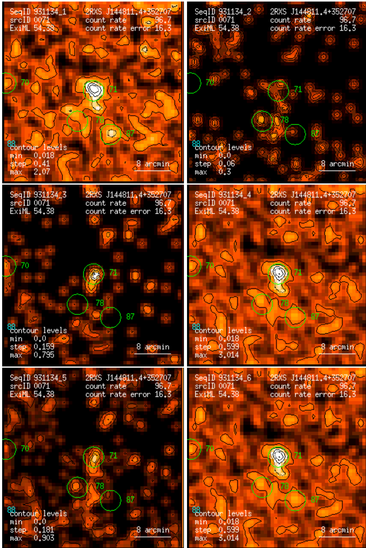
Figure 71: RASS 931134: detection 0071: band rate images, Gaussian filter: (1) PSPC channels 11 – 41, (2) 52 – 90, (3) 91 – 201, (4) 11 – 235, (5) 52 – 201, (6) 11 – 201. Broad band rates in counts/ks. Band rate contour levels in counts/ks/arcmin 2 .
