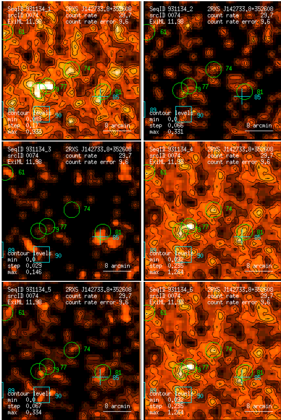
Figure 74: RASS 931134: detection 0074: band rate images, Gaussian filter: (1) PSPC channels 11 – 41, (2) 52 – 90, (3) 91 – 201, (4) 11 – 235, (5) 52 – 201, (6) 11 – 201. Broad band rates in counts/ks. Band rate contour levels in counts/ks/arcmin 2 .
