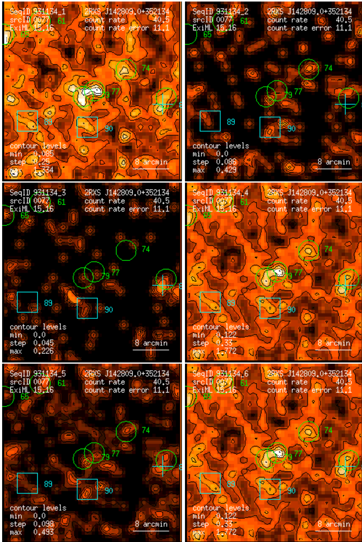
Figure 77: RASS 931134: detection 0077: band rate images, Gaussian filter: (1) PSPC channels 11 – 41, (2) 52 – 90, (3) 91 – 201, (4) 11 – 235, (5) 52 – 201, (6) 11 – 201. Broad band rates in counts/ks. Band rate contour levels in counts/ks/arcmin 2 .
