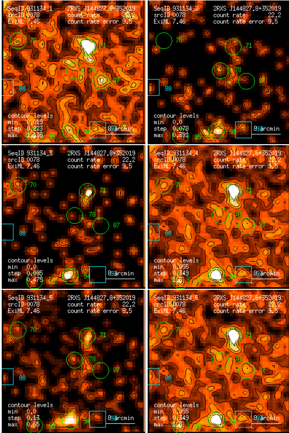
Figure 78: RASS 931134: detection 0078: band rate images, Gaussian filter: (1) PSPC channels 11 – 41, (2) 52 – 90, (3) 91 – 201, (4) 11 – 235, (5) 52 – 201, (6) 11 – 201. Broad band rates in counts/ks. Band rate contour levels in counts/ks/arcmin 2 .
