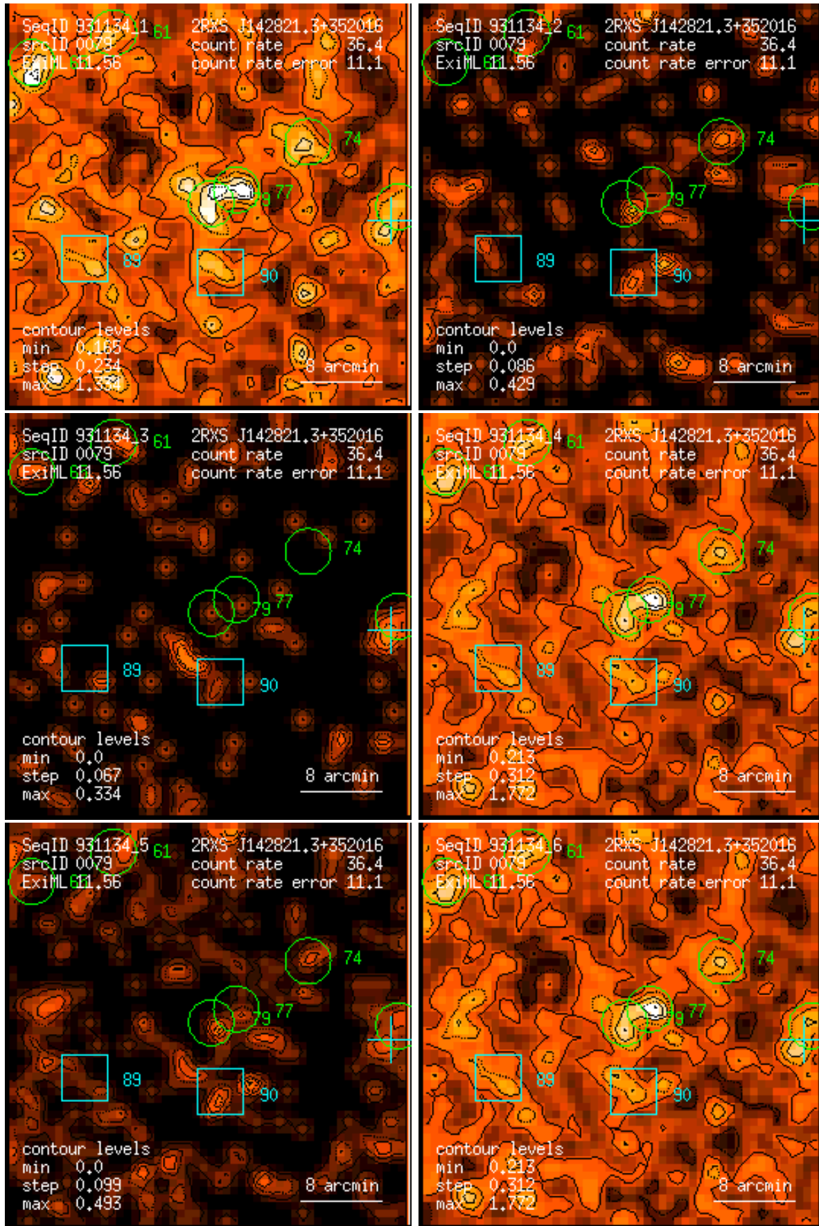
Figure 79: RASS 931134: detection 0079: band rate images, Gaussian filter: (1) PSPC channels 11 – 41, (2) 52 – 90, (3) 91 – 201, (4) 11 – 235, (5) 52 – 201, (6) 11 – 201. Broad band rates in counts/ks. Band rate contour levels in counts/ks/arcmin 2 .
