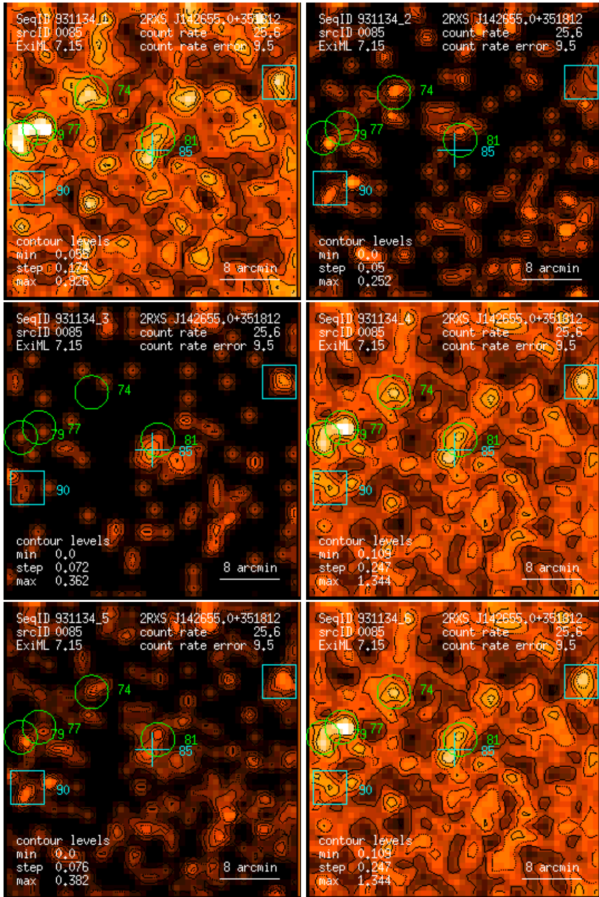
Figure 85: RASS 931134: detection 0085: band rate images, Gaussian filter: (1) PSPC channels 11 – 41, (2) 52 – 90, (3) 91 – 201, (4) 11 – 235, (5) 52 – 201, (6) 11 – 201. Broad band rates in counts/ks. Band rate contour levels in counts/ks/arcmin 2 .
