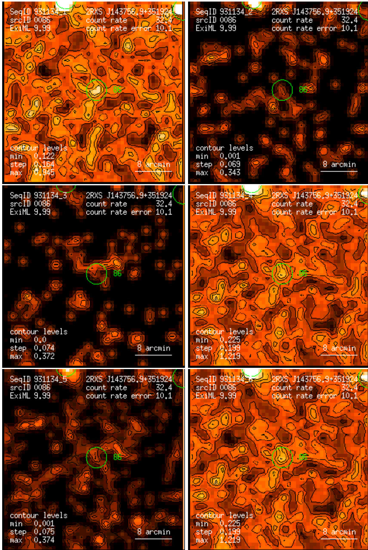
Figure 86: RASS 931134: detection 0086: band rate images, Gaussian filter: (1) PSPC channels 11 – 41, (2) 52 – 90, (3) 91 – 201, (4) 11 – 235, (5) 52 – 201, (6) 11 – 201. Broad band rates in counts/ks. Band rate contour levels in counts/ks/arcmin 2 .
