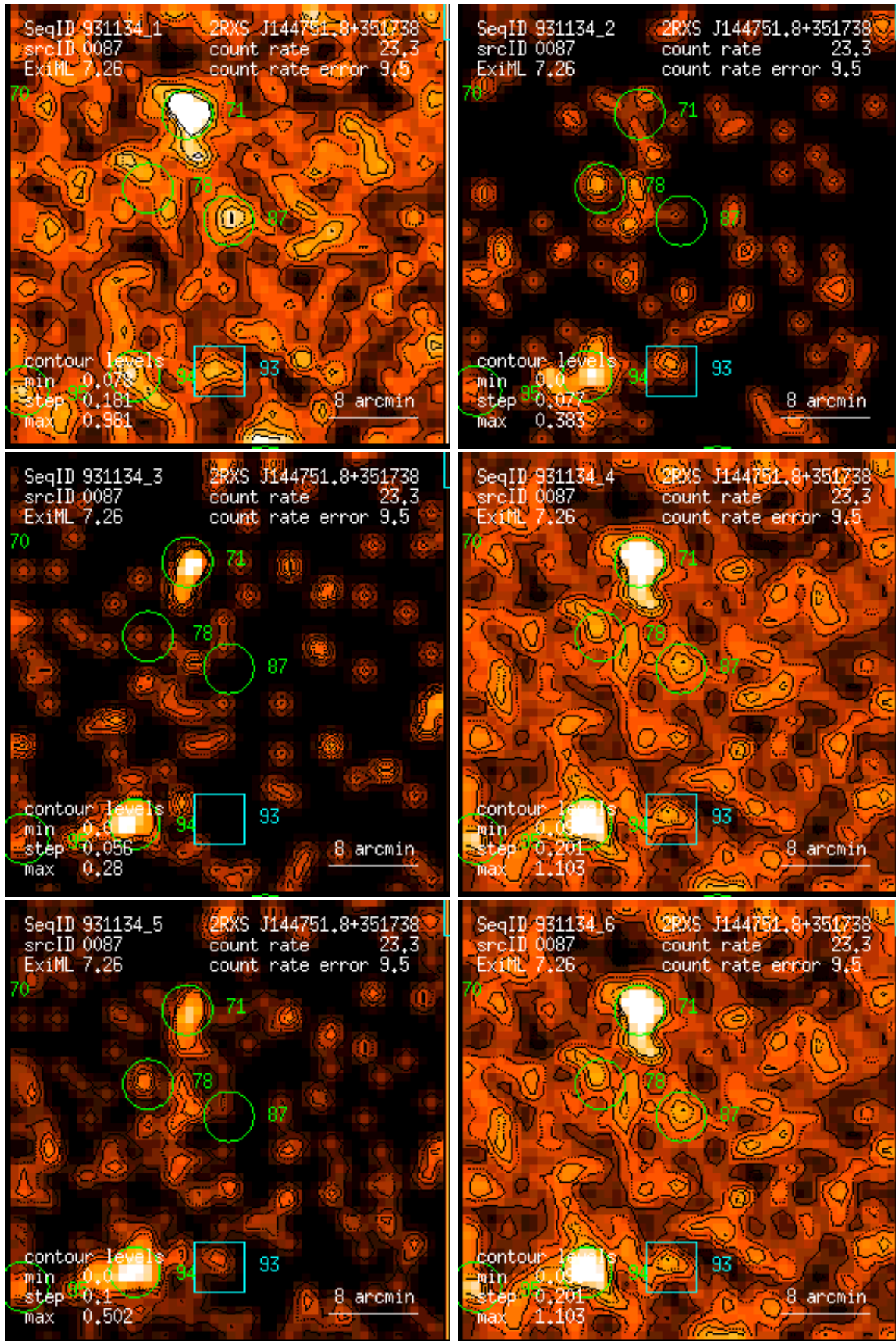
Figure 87: RASS 931134: detection 0087: band rate images, Gaussian filter: (1) PSPC channels 11 – 41, (2) 52 – 90, (3) 91 – 201, (4) 11 – 235, (5) 52 – 201, (6) 11 – 201. Broad band rates in counts/ks. Band rate contour levels in counts/ks/arcmin 2 .
