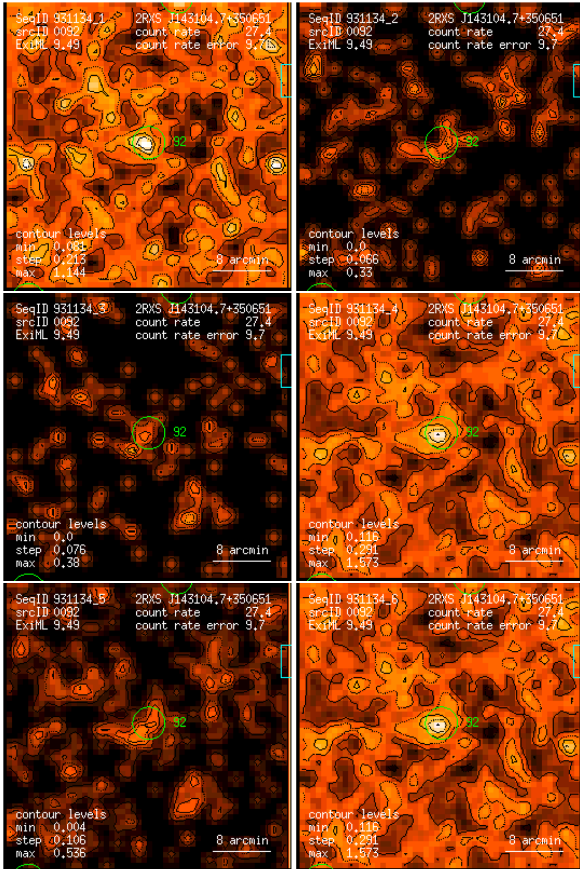
Figure 92: RASS 931134: detection 0092: band rate images, Gaussian filter: (1) PSPC channels 11 – 41, (2) 52 – 90, (3) 91 – 201, (4) 11 – 235, (5) 52 – 201, (6) 11 – 201. Broad band rates in counts/ks. Band rate contour levels in counts/ks/arcmin 2 .
