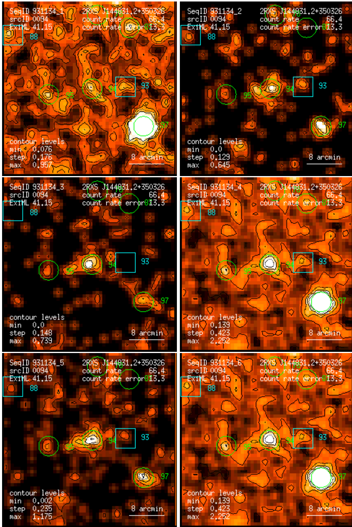
Figure 94: RASS 931134: detection 0094: band rate images, Gaussian filter: (1) PSPC channels 11 – 41, (2) 52 – 90, (3) 91 – 201, (4) 11 – 235, (5) 52 – 201, (6) 11 – 201. Broad band rates in counts/ks. Band rate contour levels in counts/ks/arcmin 2 .
