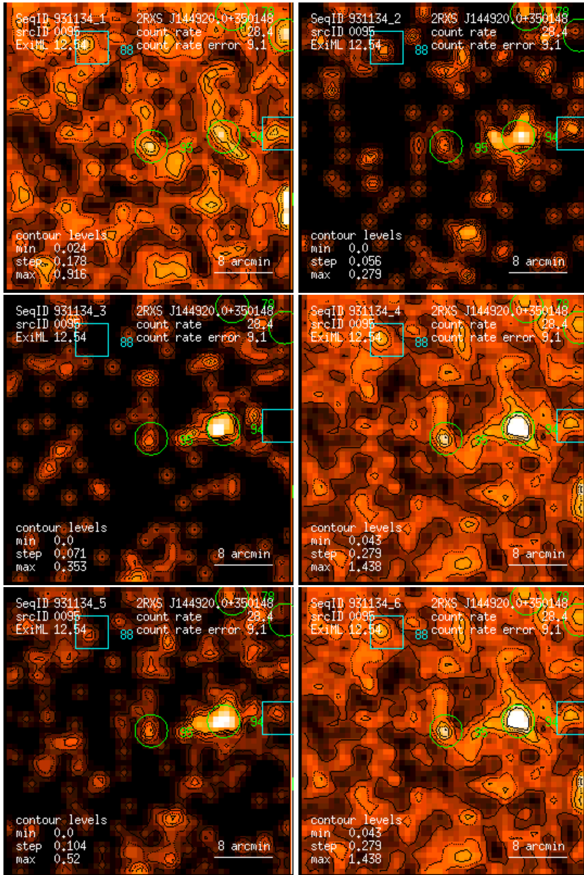
Figure 95: RASS 931134: detection 0095: band rate images, Gaussian filter: (1) PSPC channels 11 – 41, (2) 52 – 90, (3) 91 – 201, (4) 11 – 235, (5) 52 – 201, (6) 11 – 201. Broad band rates in counts/ks. Band rate contour levels in counts/ks/arcmin 2 .
