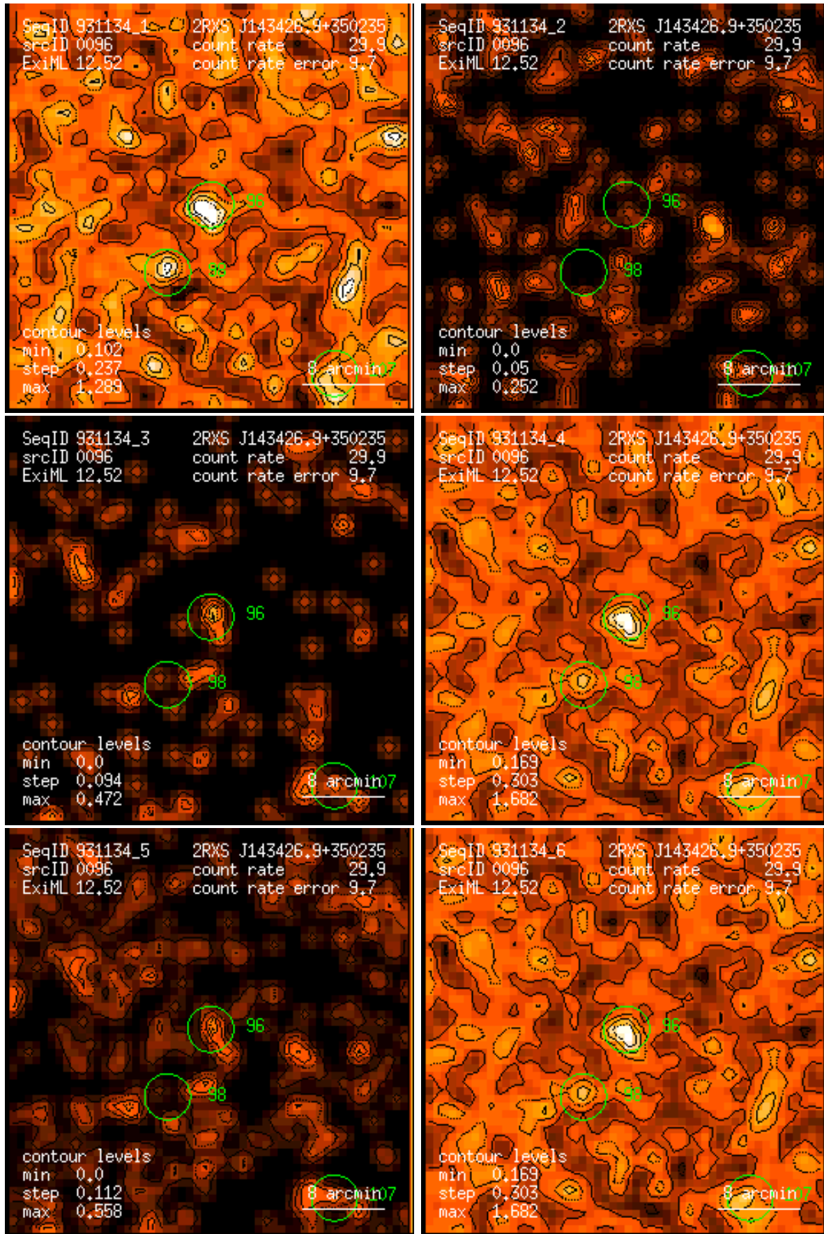
Figure 96: RASS 931134: detection 0096: band rate images, Gaussian filter: (1) PSPC channels 11 – 41, (2) 52 – 90, (3) 91 – 201, (4) 11 – 235, (5) 52 – 201, (6) 11 – 201. Broad band rates in counts/ks. Band rate contour levels in counts/ks/arcmin 2 .
