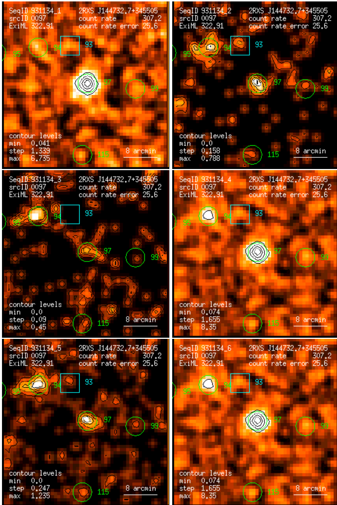
Figure 97: RASS 931134: detection 0097: band rate images, Gaussian filter: (1) PSPC channels 11 – 41, (2) 52 – 90, (3) 91 – 201, (4) 11 – 235, (5) 52 – 201, (6) 11 – 201. Broad band rates in counts/ks. Band rate contour levels in counts/ks/arcmin 2 .
