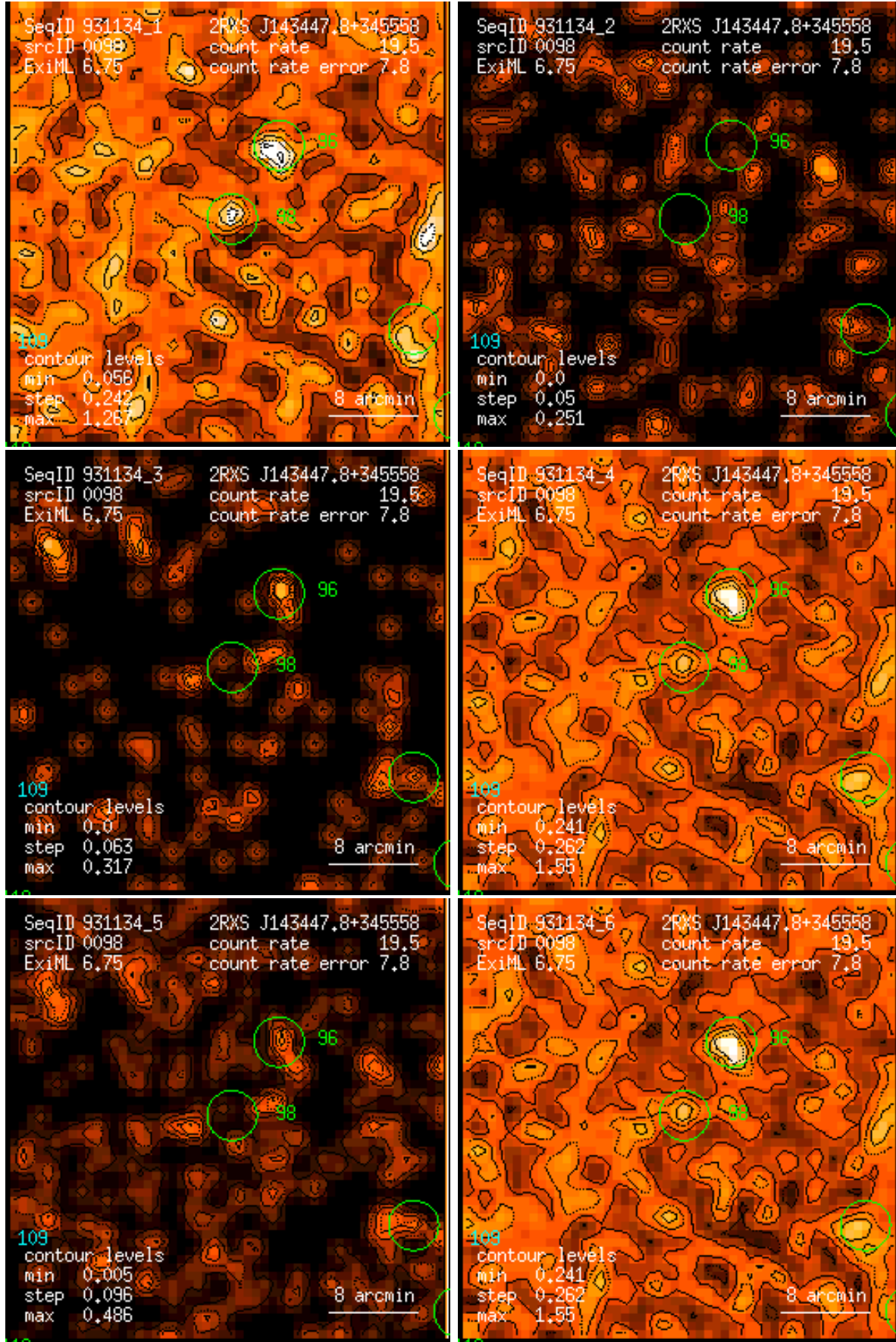
Figure 98: RASS 931134: detection 0098: band rate images, Gaussian filter: (1) PSPC channels 11 – 41, (2) 52 – 90, (3) 91 – 201, (4) 11 – 235, (5) 52 – 201, (6) 11 – 201. Broad band rates in counts/ks. Band rate contour levels in counts/ks/arcmin 2 .
