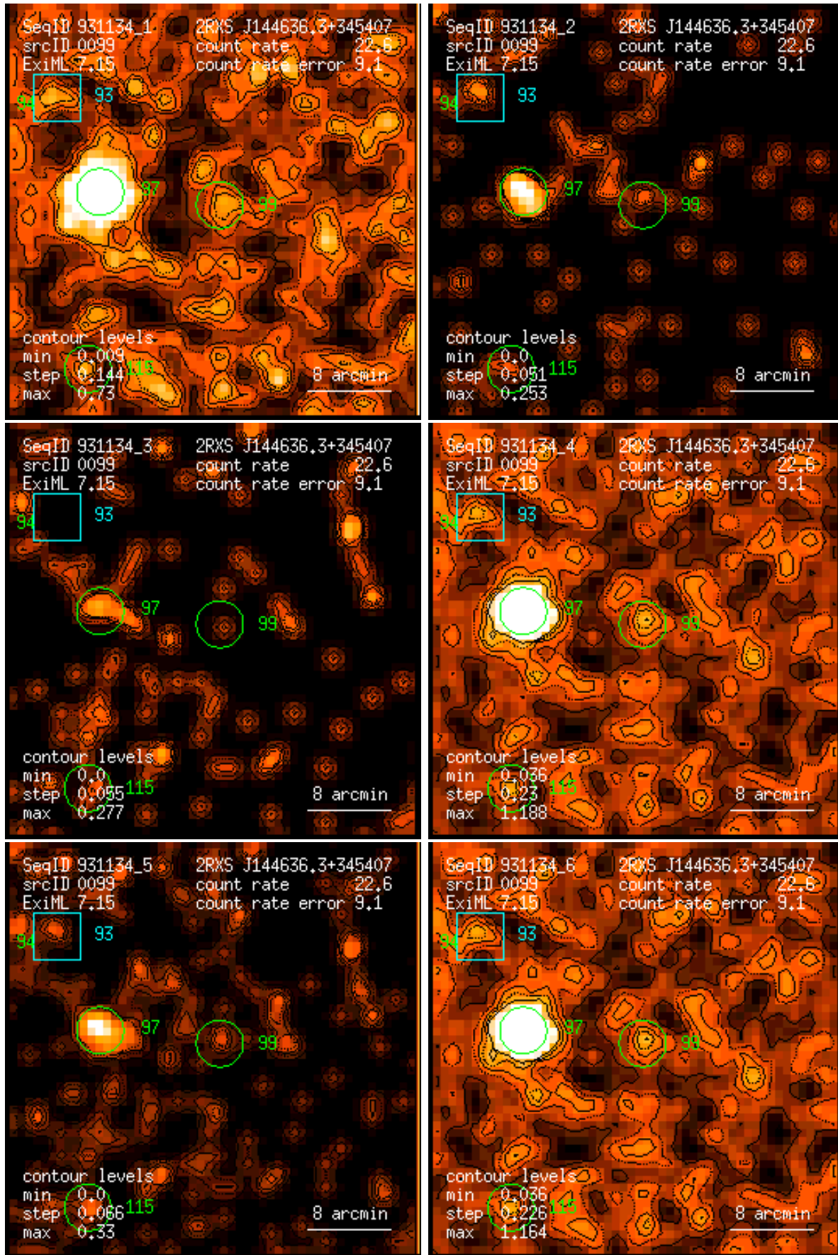
Figure 99: RASS 931134: detection 0099: band rate images, Gaussian filter: (1) PSPC channels 11 – 41, (2) 52 – 90, (3) 91 – 201, (4) 11 – 235, (5) 52 – 201, (6) 11 – 201. Broad band rates in counts/ks. Band rate contour levels in counts/ks/arcmin 2 .
