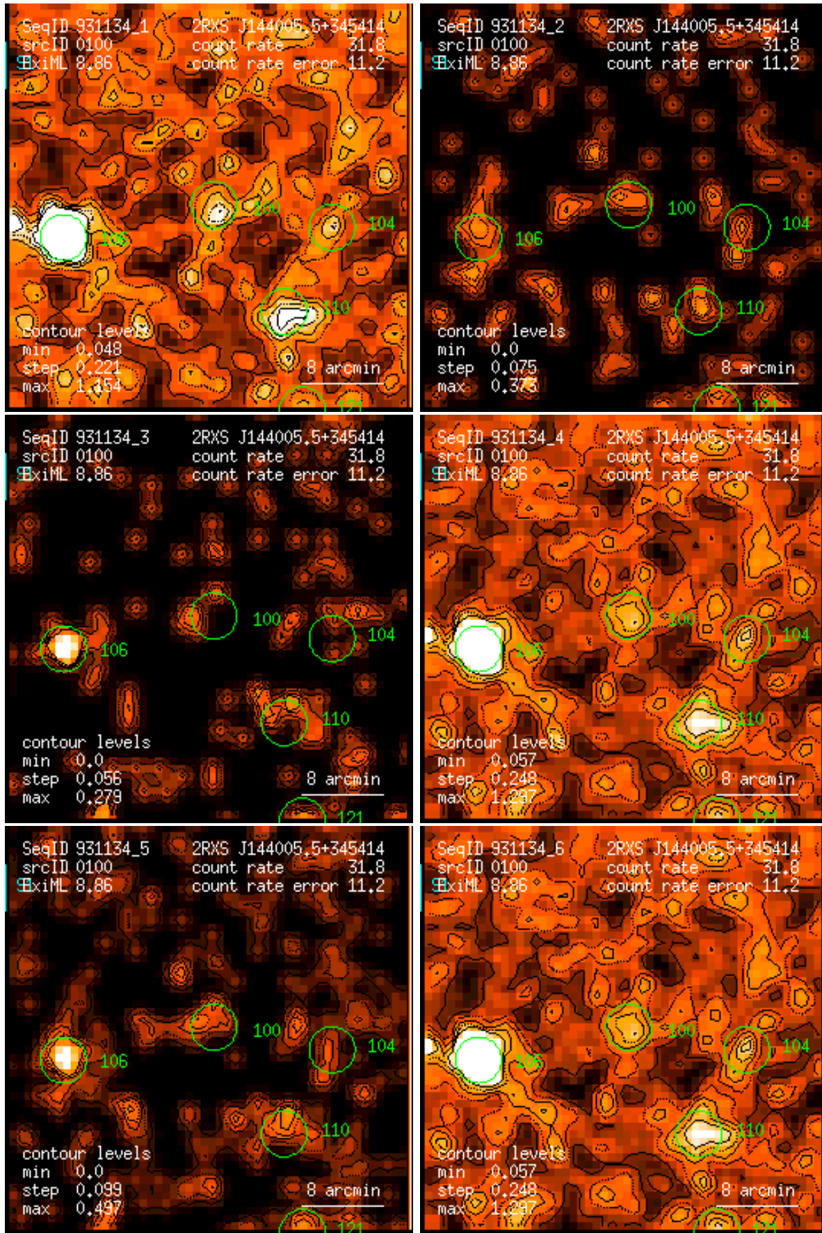
Figure 100: RASS 931134: detection 0100: band rate images, Gaussian filter: (1) PSPC channels 11 – 41, (2) 52 – 90, (3) 91 – 201, (4) 11 – 235, (5) 52 – 201, (6) 11 – 201. Broad band rates in counts/ks. Band rate contour levels in counts/ks/arcmin 2 .
