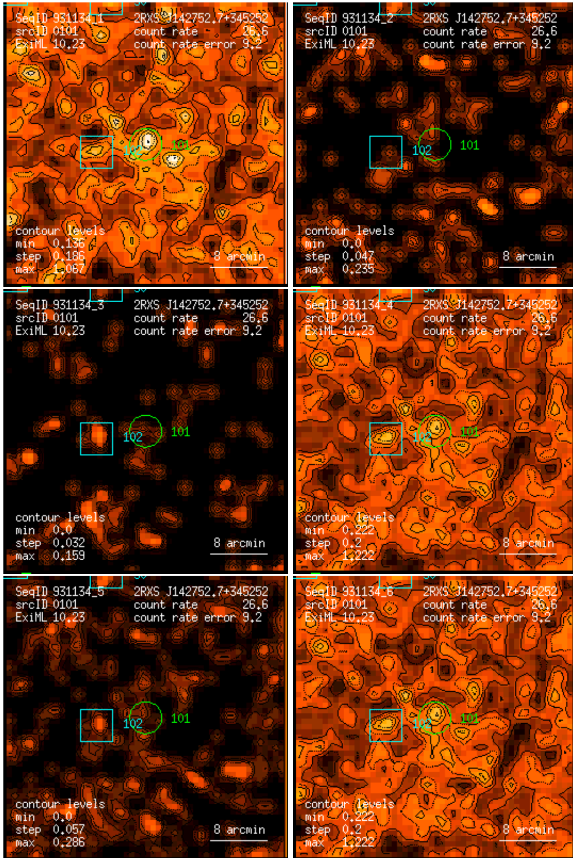
Figure 101: RASS 931134: detection 0101: band rate images, Gaussian filter: (1) PSPC channels 11 – 41, (2) 52 – 90, (3) 91 – 201, (4) 11 – 235, (5) 52 – 201, (6) 11 – 201. Broad band rates in counts/ks. Band rate contour levels in counts/ks/arcmin 2 .
