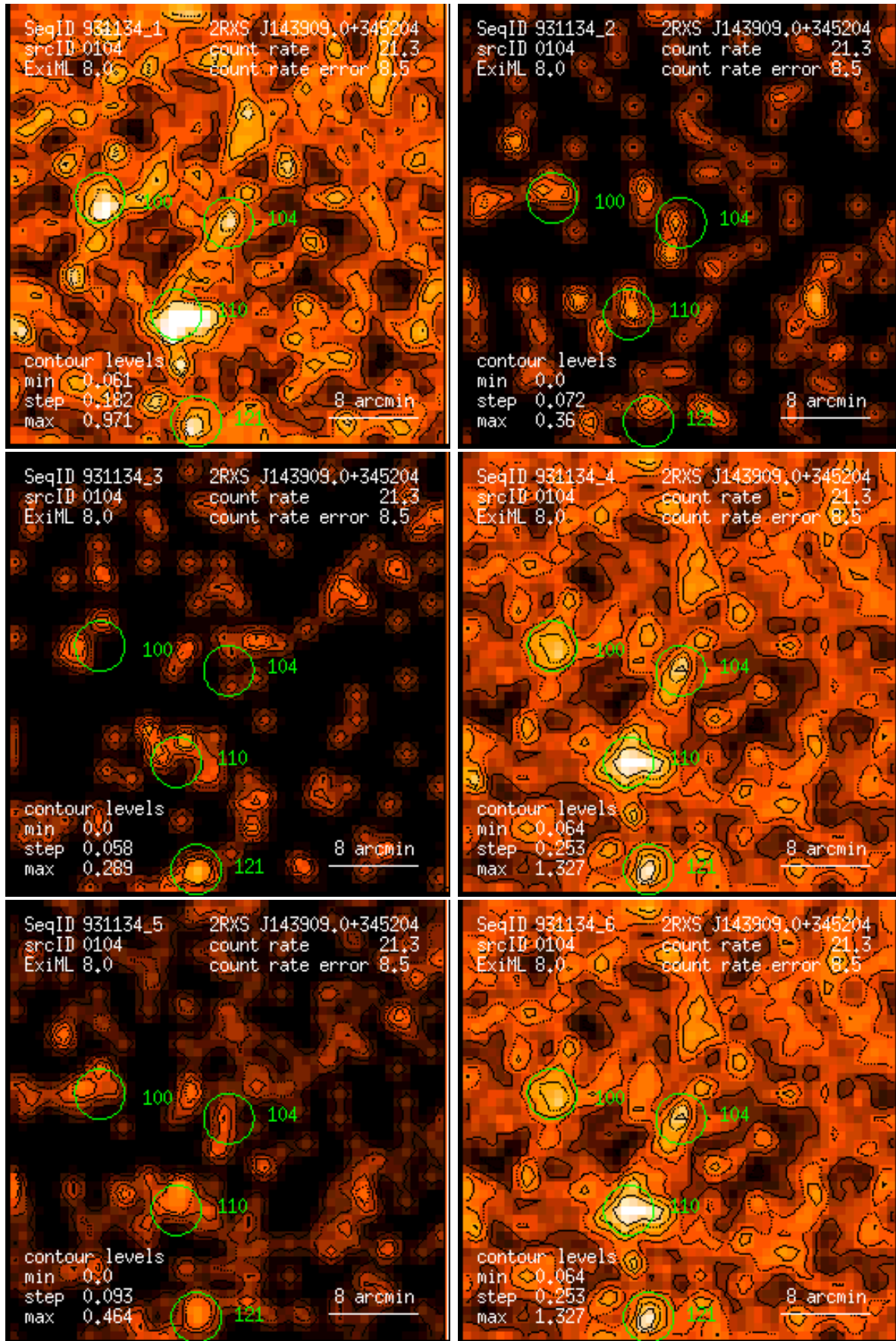
Figure 104: RASS 931134: detection 0104: band rate images, Gaussian filter: (1) PSPC channels 11 – 41, (2) 52 – 90, (3) 91 – 201, (4) 11 – 235, (5) 52 – 201, (6) 11 – 201. Broad band rates in counts/ks. Band rate contour levels in counts/ks/arcmin 2 .
