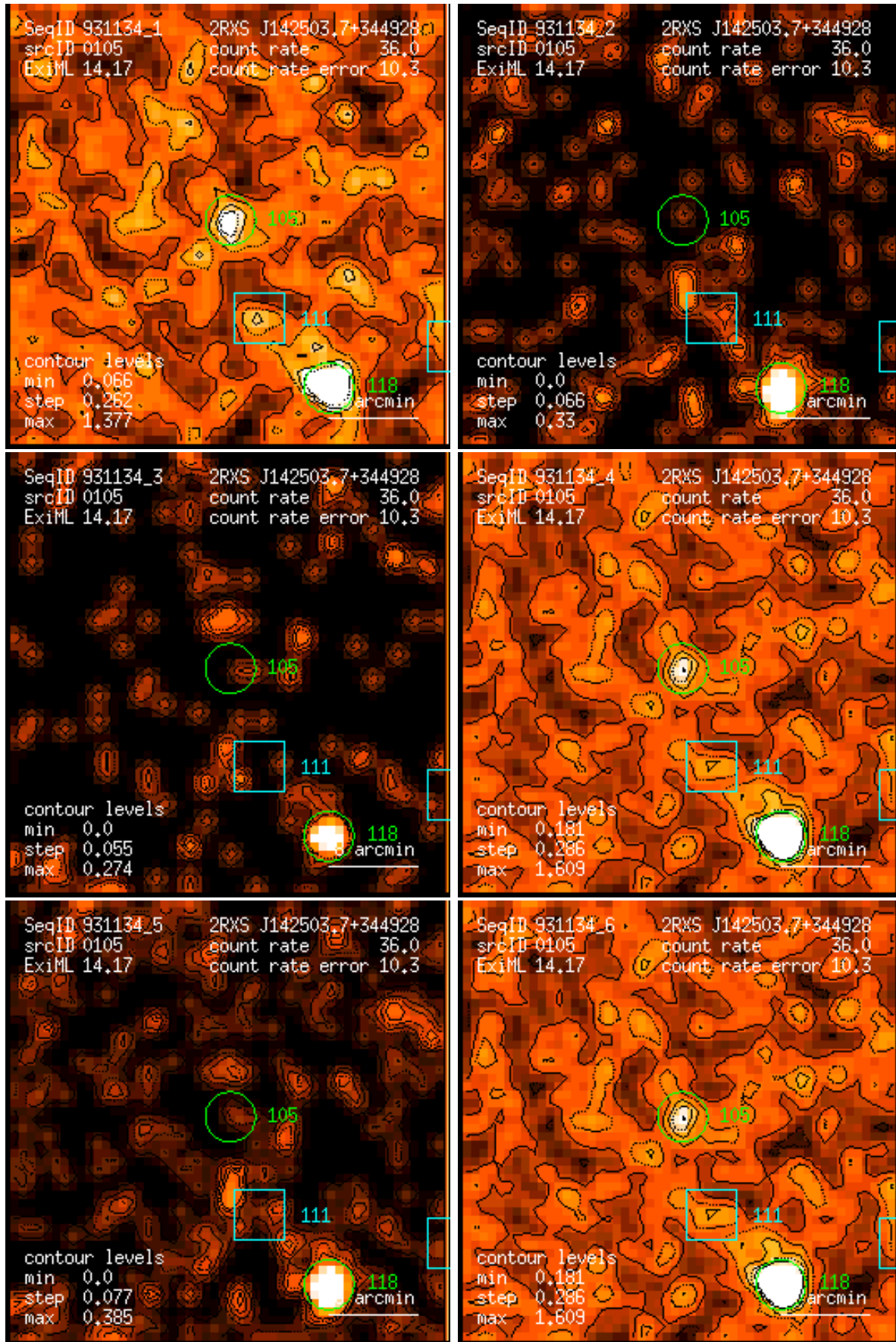
Figure 105: RASS 931134: detection 0105: band rate images, Gaussian filter: (1) PSPC channels 11 – 41, (2) 52 – 90, (3) 91 – 201, (4) 11 – 235, (5) 52 – 201, (6) 11 – 201. Broad band rates in counts/ks. Band rate contour levels in counts/ks/arcmin 2 .
