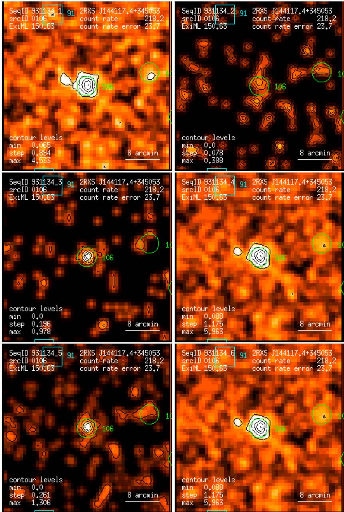
Figure 106: RASS 931134: detection 0106: band rate images, Gaussian filter: (1) PSPC channels 11 – 41, (2) 52 – 90, (3) 91 – 201, (4) 11 – 235, (5) 52 – 201, (6) 11 – 201. Broad band rates in counts/ks. Band rate contour levels in counts/ks/arcmin 2 .
