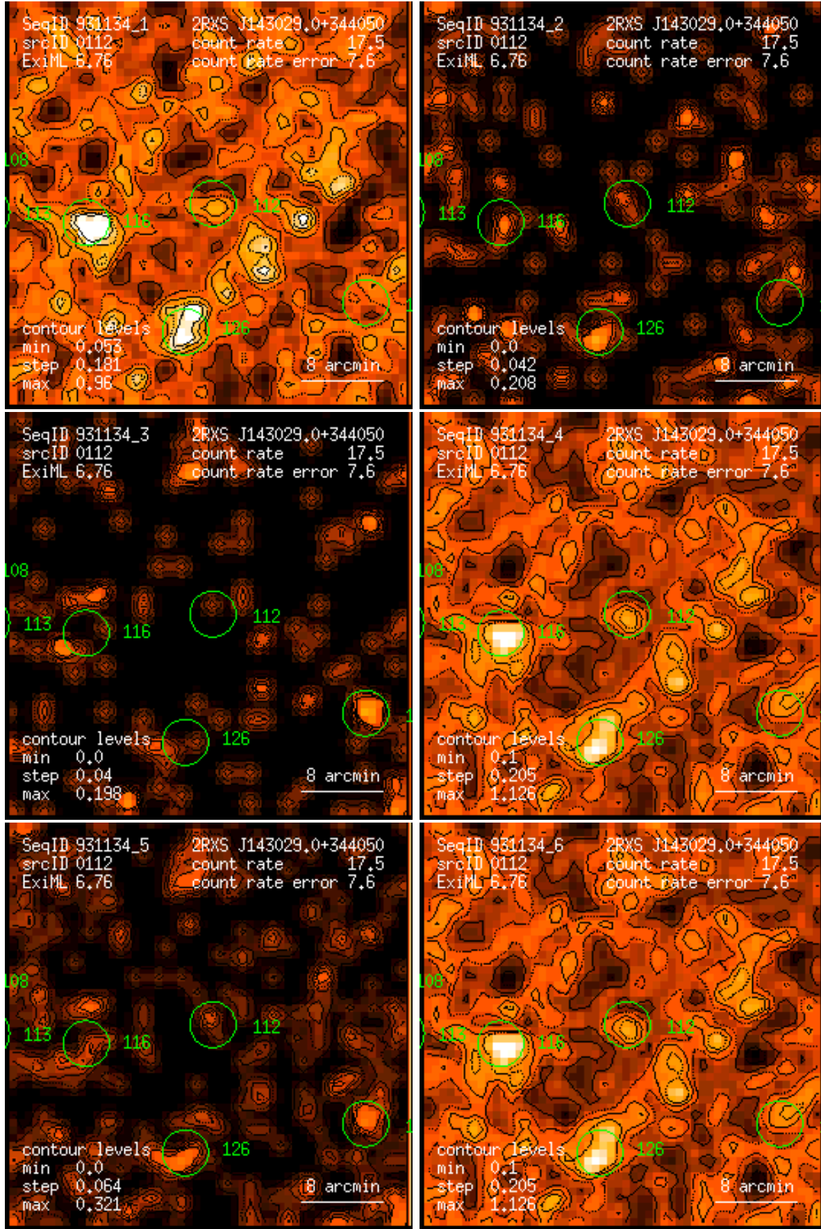
Figure 112: RASS 931134: detection 0112: band rate images, Gaussian filter: (1) PSPC channels 11 – 41, (2) 52 – 90, (3) 91 – 201, (4) 11 – 235, (5) 52 – 201, (6) 11 – 201. Broad band rates in counts/ks. Band rate contour levels in counts/ks/arcmin 2 .
