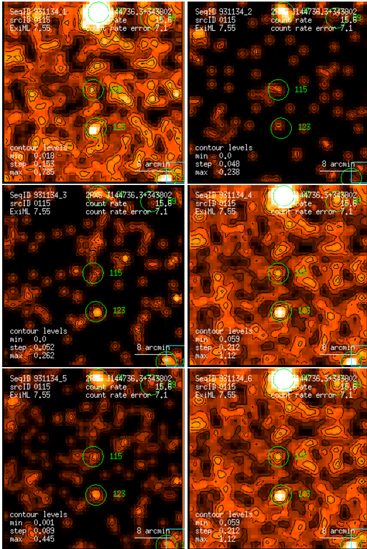
Figure 115: RASS 931134: detection 0115: band rate images, Gaussian filter: (1) PSPC channels 11 – 41, (2) 52 – 90, (3) 91 – 201, (4) 11 – 235, (5) 52 – 201, (6) 11 – 201. Broad band rates in counts/ks. Band rate contour levels in counts/ks/arcmin 2 .
