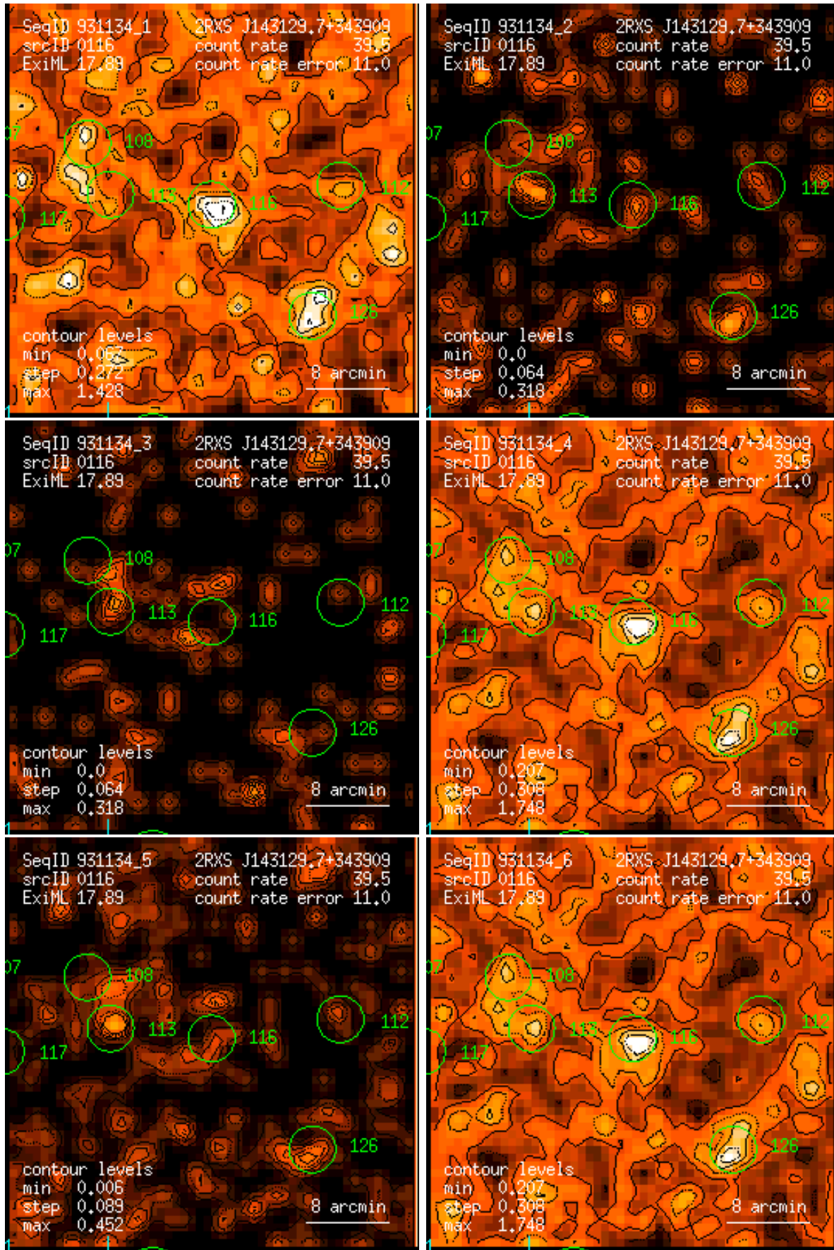
Figure 116: RASS 931134: detection 0116: band rate images, Gaussian filter: (1) PSPC channels 11 – 41, (2) 52 – 90, (3) 91 – 201, (4) 11 – 235, (5) 52 – 201, (6) 11 – 201. Broad band rates in counts/ks. Band rate contour levels in counts/ks/arcmin 2 .
