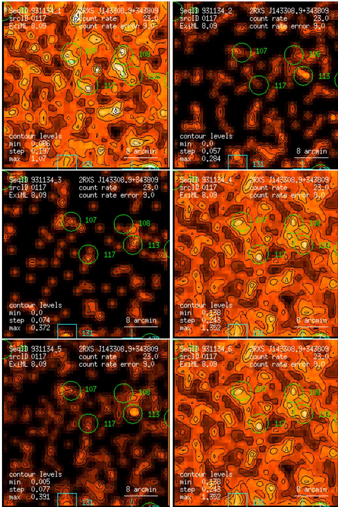
Figure 117: RASS 931134: detection 0117: band rate images, Gaussian filter: (1) PSPC channels 11 – 41, (2) 52 – 90, (3) 91 – 201, (4) 11 – 235, (5) 52 – 201, (6) 11 – 201. Broad band rates in counts/ks. Band rate contour levels in counts/ks/arcmin 2 .
